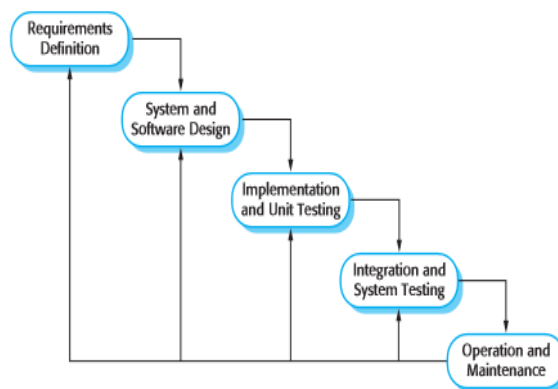
Gambar 1. Waterfall Sommerville
