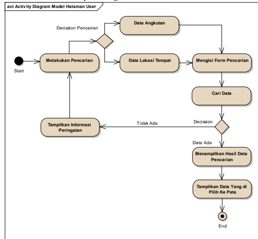
Gambar 3. Activity Diagram Halaman User
