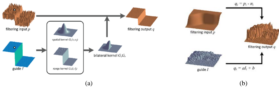
Figure 3: (a) Bilateral Filter Process and (b) Guided Filter Process
