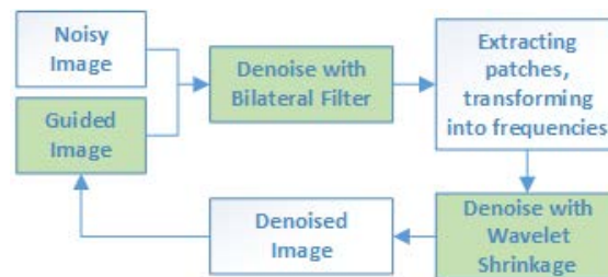
Figure 7: Dual Domain Image Denoising process
