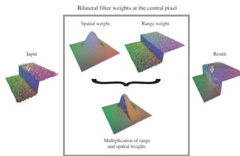
Figure 1: Bilateral filter for smoothing an input image [3]
