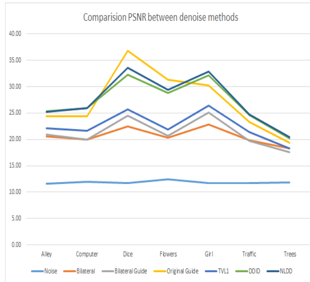
Figure10: Comparison PSNR between denoise methods
