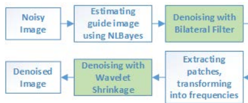
Figure 8: Non-local dual denoising process
