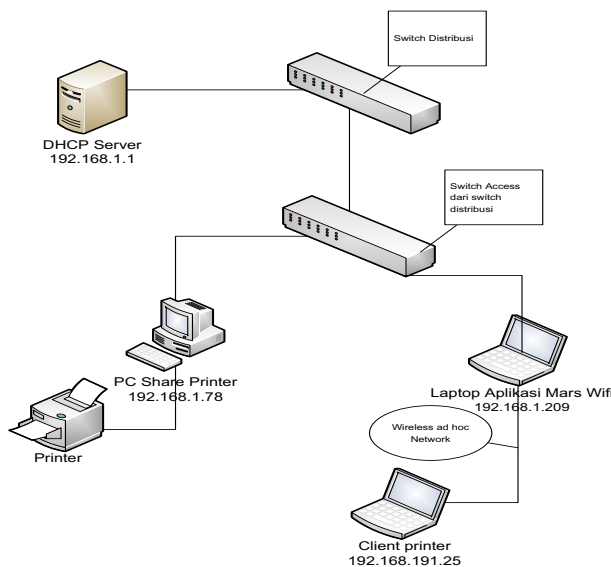
Gambar 6 Topologi Share Printer
