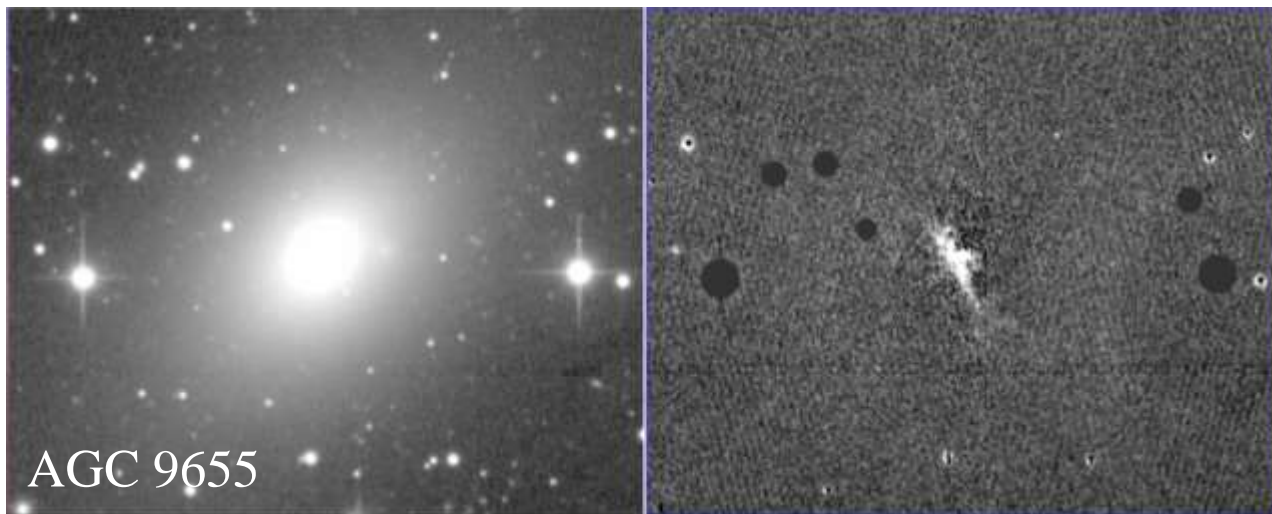
Image Reduced by Warren, M. Union College Summer Research Paper Note that AGC 9655 appears to have some sort of outflow, possibly AGN activity.
