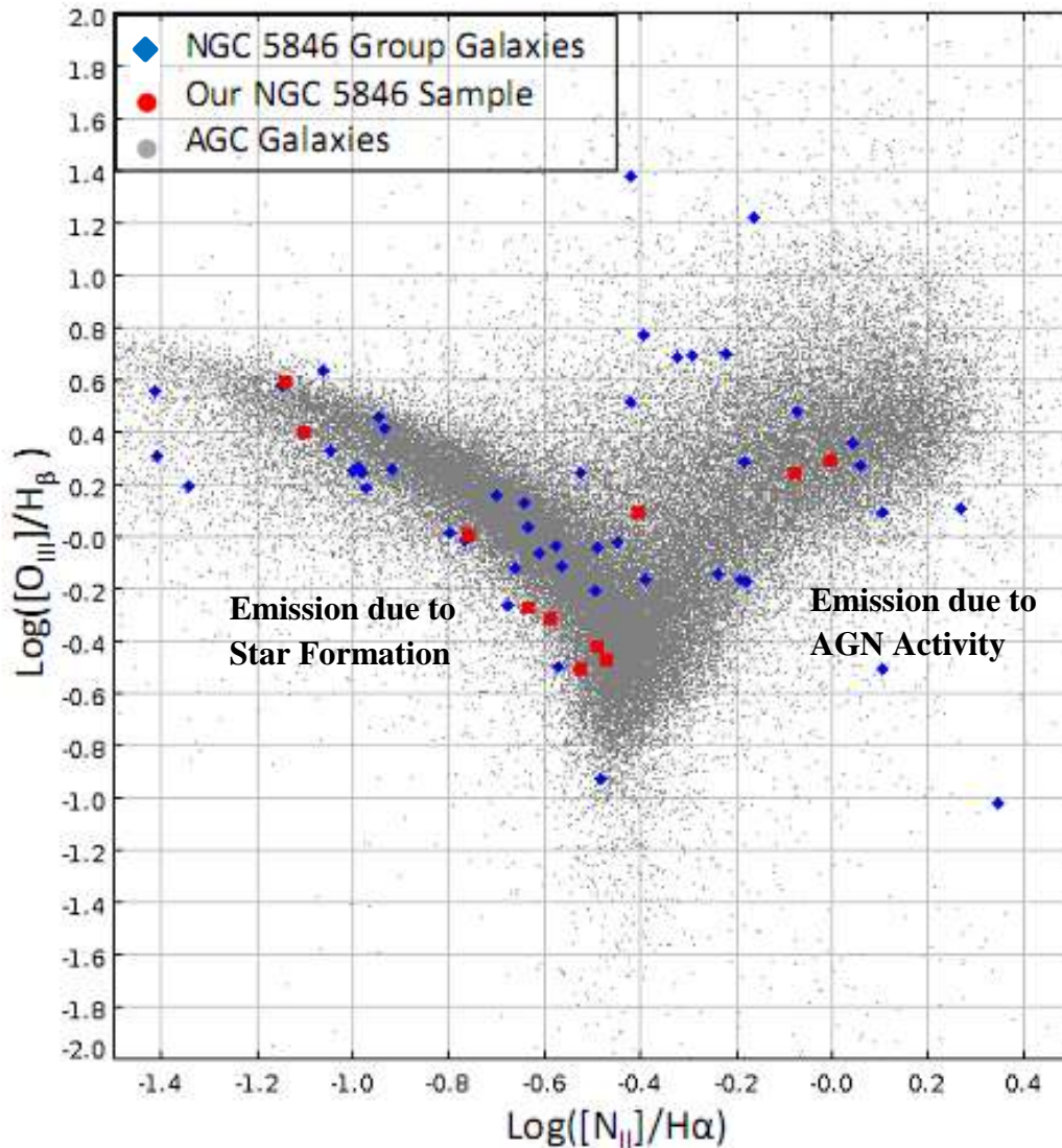
Figure 14: A BPT (Baldwin, Phillips, & Terlevich) diagram for NGC 5846 galaxies (blue), our NGC 5846 sample (red), and other AGC galaxies (grey). BPT diagrams compare the ratios [O_{III}]/H_{\beta} and [N_{II}]/H_{\alpha} . Star forming galaxies fall on the left side of the plot and galaxies with emission due to AGN fall on the right side of the plot. Most of the galaxies with global star-forming activity also have ionization due to star formation in their nuclei.
