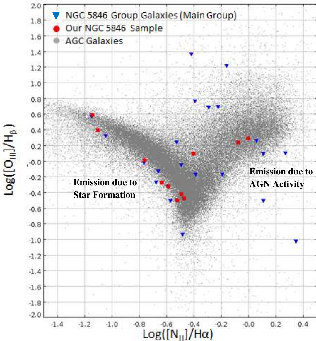
Figure 15: A BPT diagram of our NGC 5846 sample (red), the rest of the main group region of NGC 5846 (blue), and other AGC galaxies (grey). Galaxies on the left side of the “sea-gull” pattern have emission due to star formation activity and galaxies on the right have emission due to AGN activity. Comparing to Figure 14 it is evident that the main group region of NGC 5846 has less star forming galaxies than the outskirts of the group.
