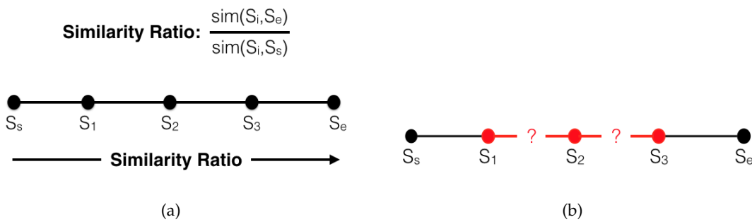
Figure 16: The Start-End algorithm allows similarity to change without a change in similarity ratio.
