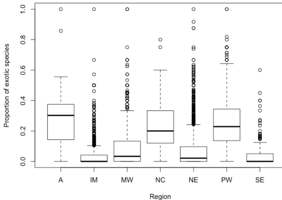
Figure 3: ANOVA of proportion of exotic species vs. region. (A-Alaska, IM-Intermountain, MW-Midwest, NC-Nations Capital, NE-Northeast, PW-Pacific West, SE-Southeast).
