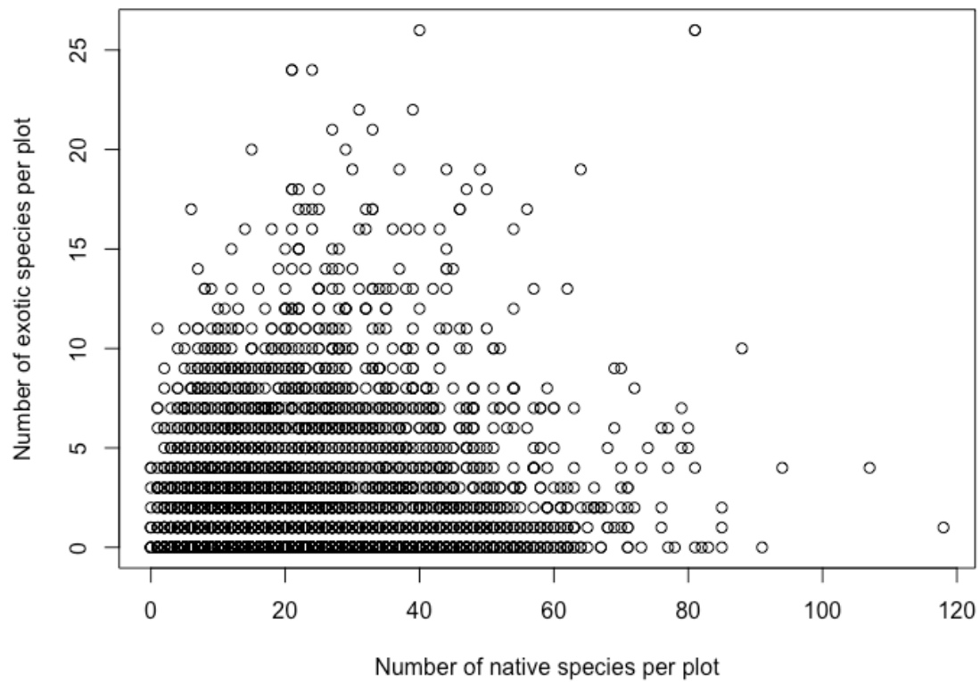
Figure 1: Correlation between native species richness and exotic species richness per plot.
