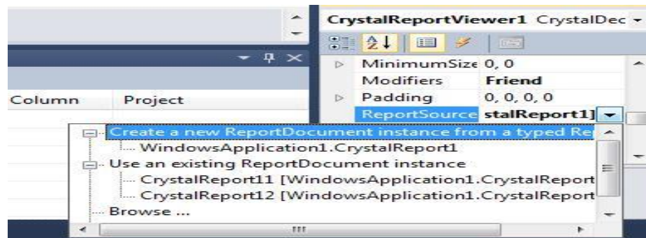
Gambar 21 : Report Sources
