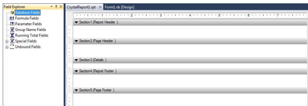
Gambar 16 : Crystall Reports
