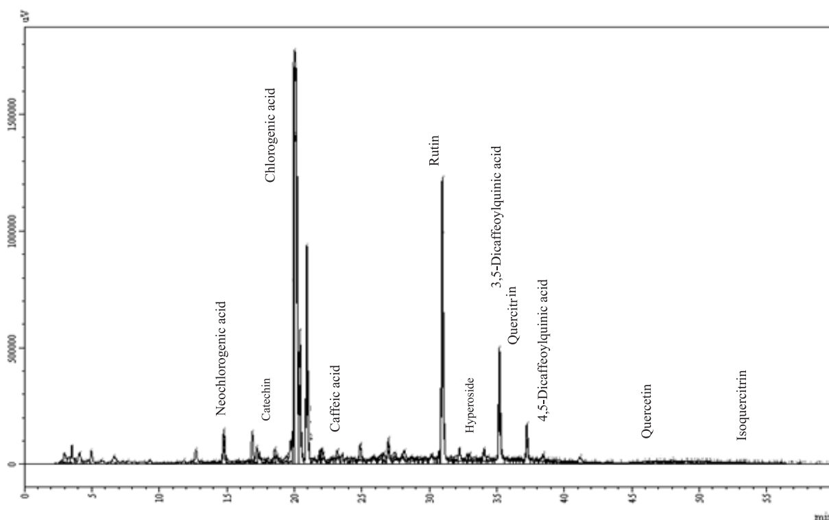
Fig. The typical chromatogram of phenolic compounds of the liquid alcohol extract from cleavers herb
