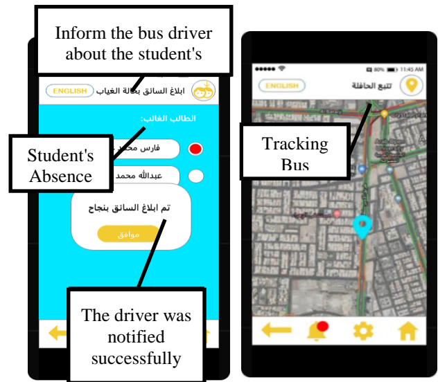
Figure 6: Informing the bus driver and tracking the bus
