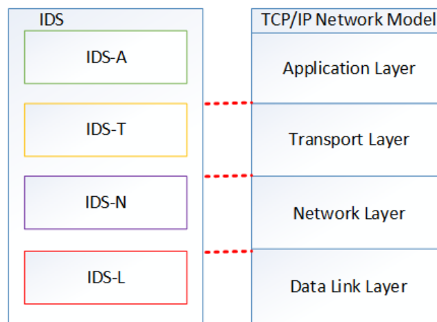
Fig. 3. NIDS architecture [15]
