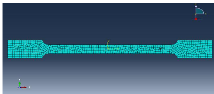
Figure 10: Mesh of the specimen
