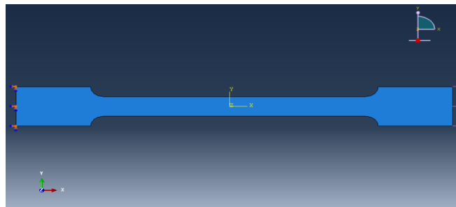
Figure 9: Boundary conditions and loading
