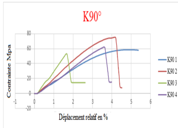
Figure 7: Tensile curves at 90^\circ [4]
