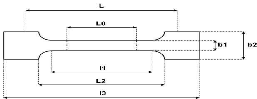
Figure 1: Normalized specimen
