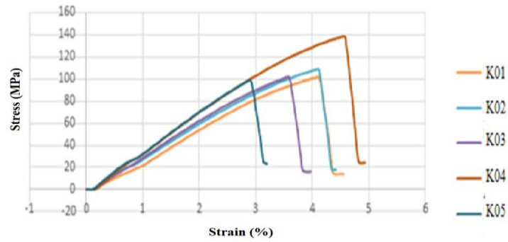
Figure 3: Tensile curves at 0° [4]
