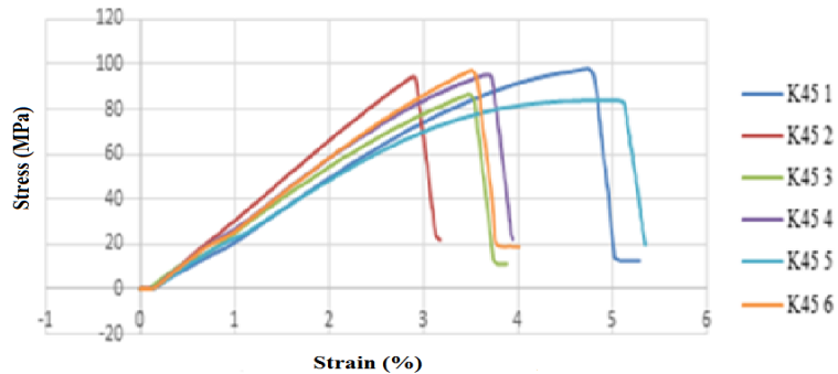
Figure 5: Tensile curves at 45° [4]
