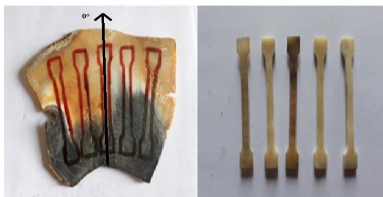
Figure 2: Cutting specimens parallel to the fibers [4]
