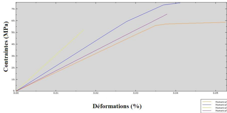
Figure 11: Numerical stress-strain curves at 90^\circ of fiber direction
