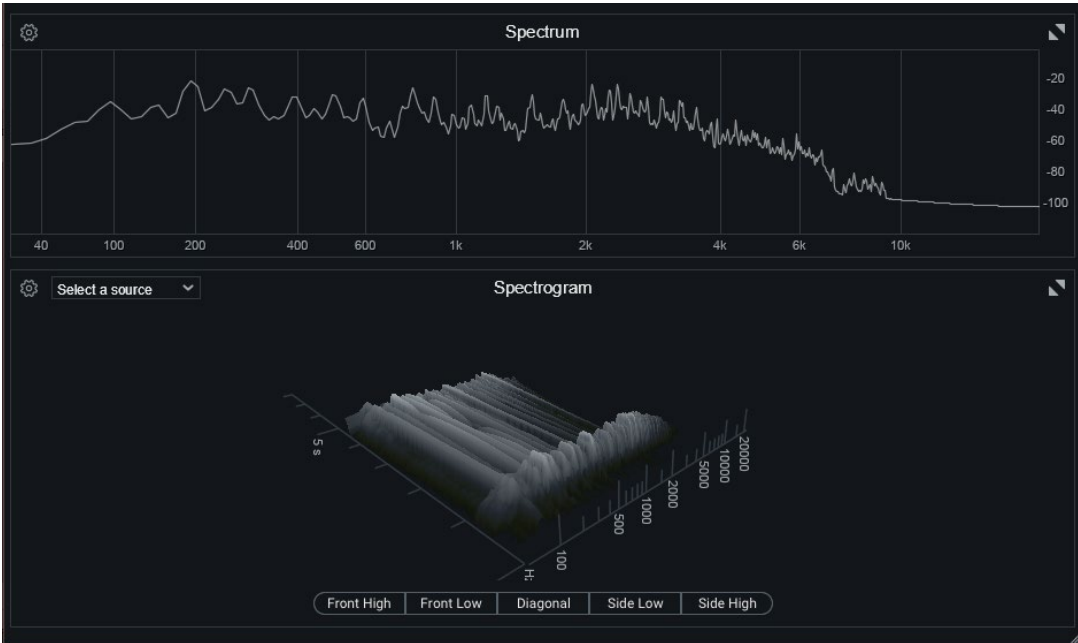
Fig. 2: Spectral Analysis of Custom Cabinet
