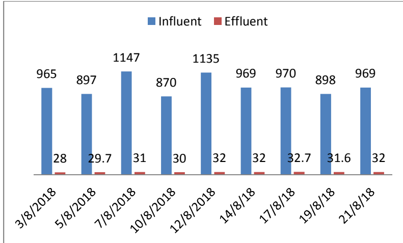
Fig. 7: (Chemical Oxygen Demand) Influent and Effluent Reading for Raining Season (mg/l).
