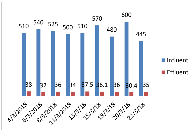
Fig.2: (Bio Chemical Oxygen Demand) Influent and Effluent Reading for Dry Season. (mg/l).
