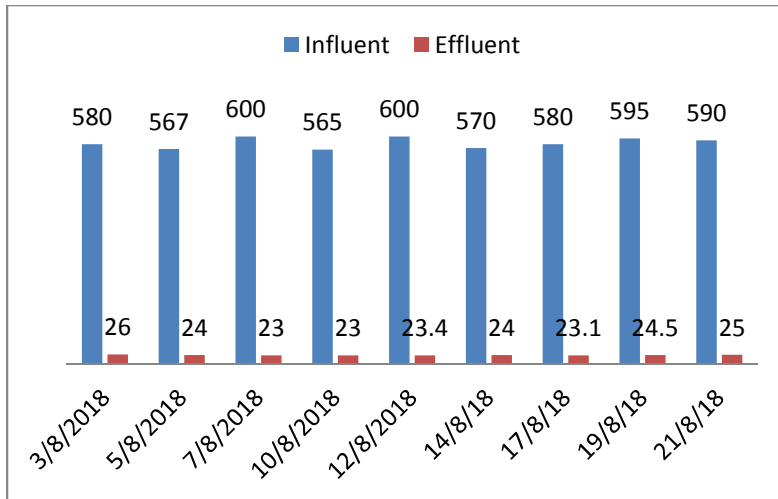
Fig. 5: (Total Suspended Solids) Influent and Effluent Reading for Raining Season (ppm).
