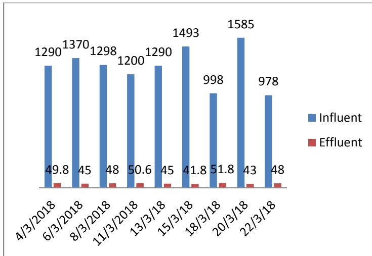
Fig. 3: Chemical Oxygen Demand) Influent and Effluent Reading for Dry Season (mg/l).
