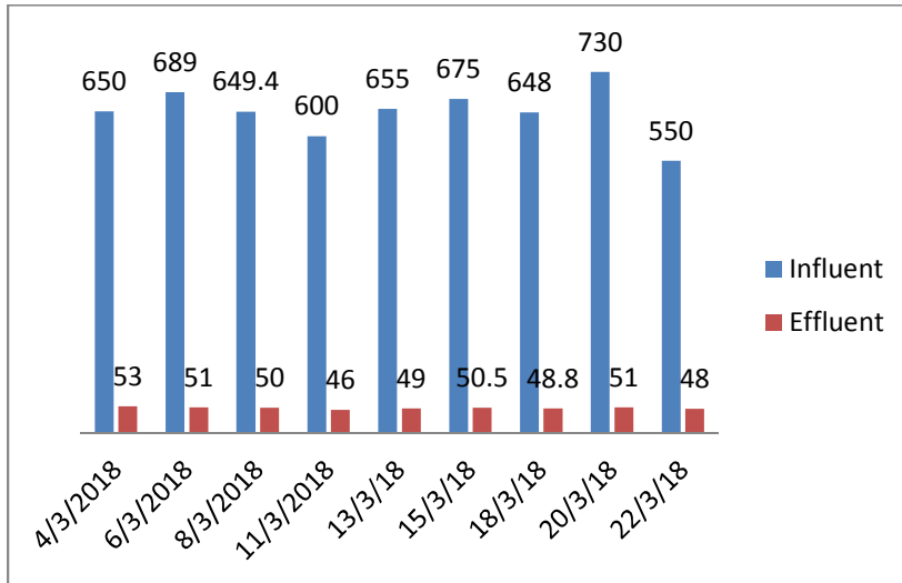
Fig. 1: (Total Suspended Solids); The Influent and Effluent Reading for Dry Season (ppm).
