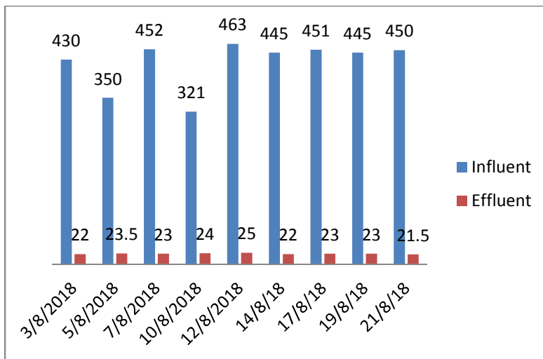
Fig. 6: (Biological Oxygen Demand) Influent and Effluent Reading for Raining Season. (mg/l).
