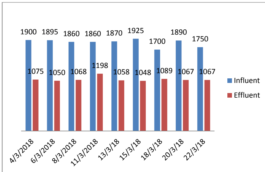
Fig. 4: (Total Dissolved Solid) influent and effluent reading for dry season (ppm).
