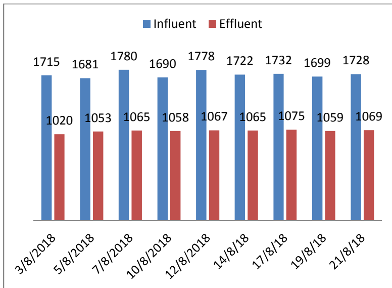
Fig. 8: (Total Dissolved Solid) Influent and Effluent Reading for Dry Season (ppm).
