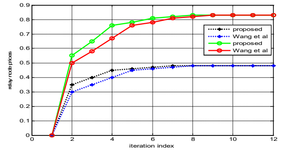
Fig. 6 Plots comparing the convergence speeds of the proposed game scheme with the scheme in Wang et al [1] for a 2-relay node network
