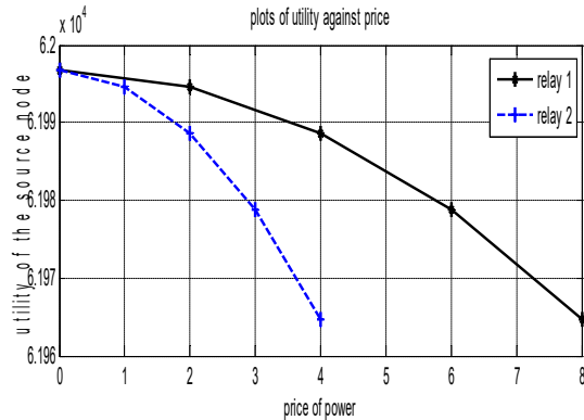
Fig. 3 Plots showing the variation of the source utility with the unit price of power
