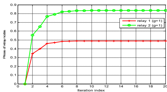
Fig. 5 Observance of convergence speed using the relay node's prices versus iteration index, with two relay nodes in the system
