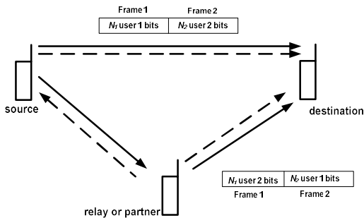
Fig.1 A 3 – node coded cooperative communication scheme
