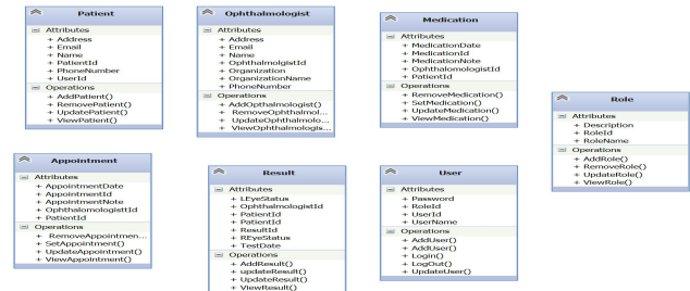
Fig. 3.2: The Class Diagram
