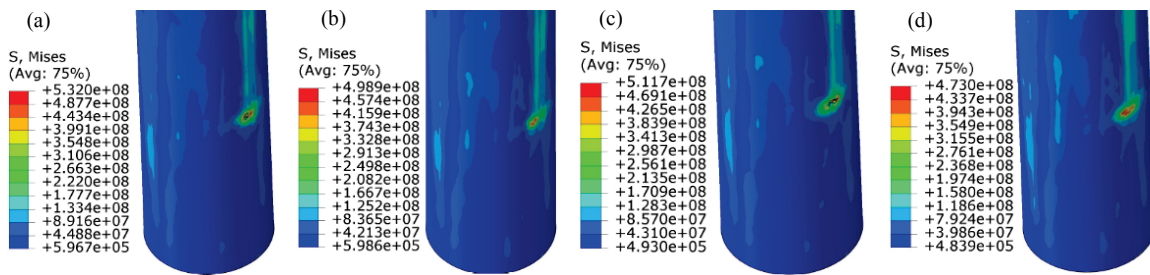
Fig. 10 – von-Mises stresses in pole by (a) 600 (b) 1200 (c) 1800 and (d) 2400 kg speed at 5 ms.
