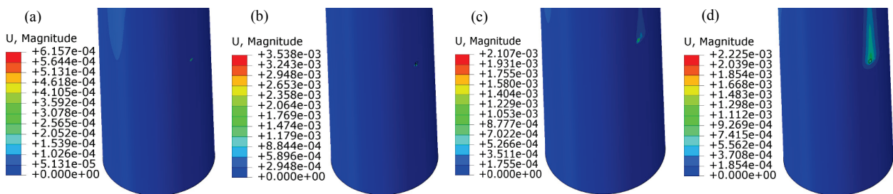
Fig. 8 – Deflection (m) of pole against (a) 40 (b) 80 (c) 120 and (d) 160 kmph speed at 5 ms.
