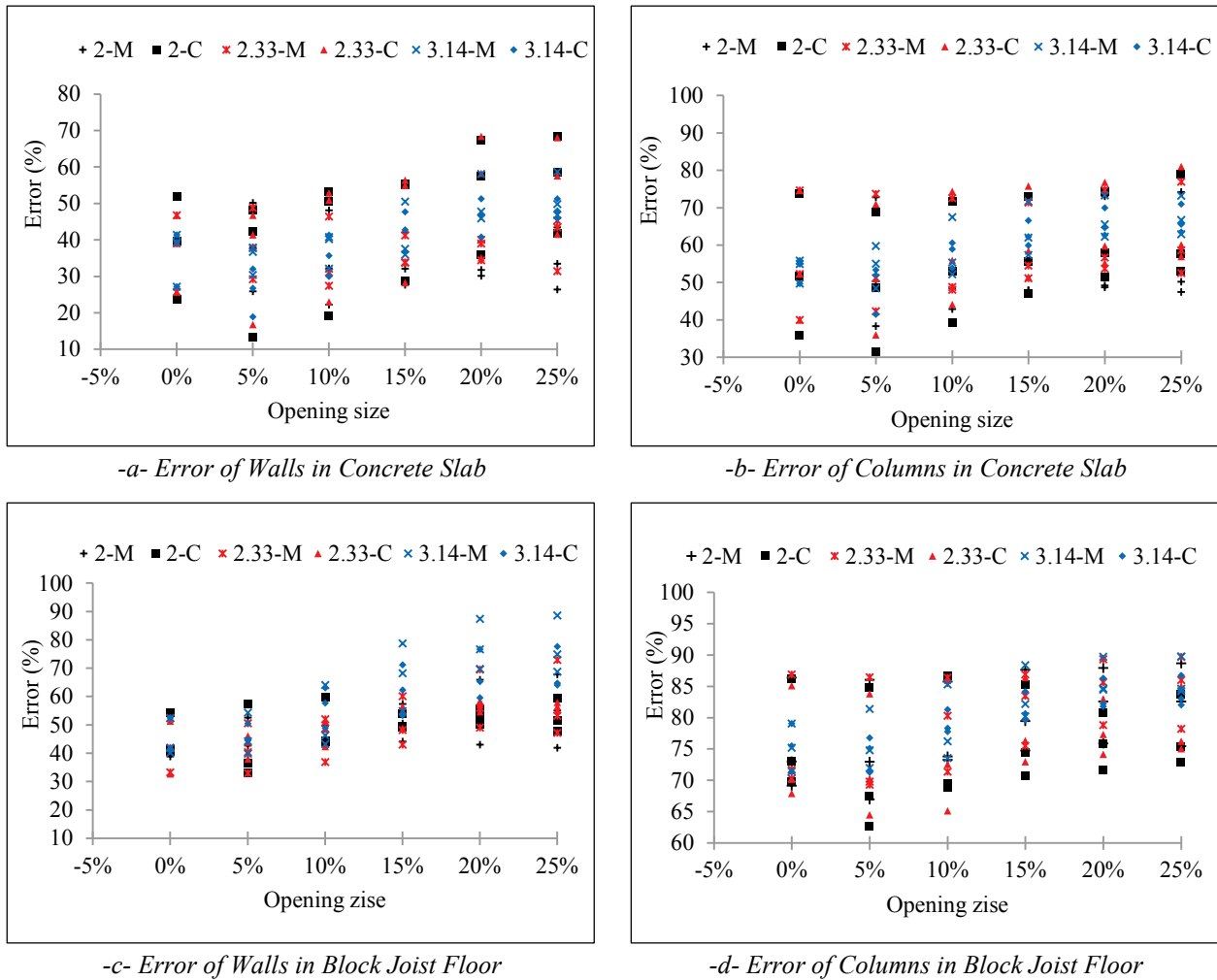
Figure 3- Shear Force Error in Vertical Resisting Elements.
