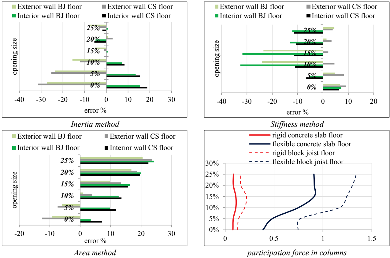
Figure 6- Error of distribution horizontal forces in shear wall for position 3 ratio 2 flexible diaphragms (opening located in middle)
