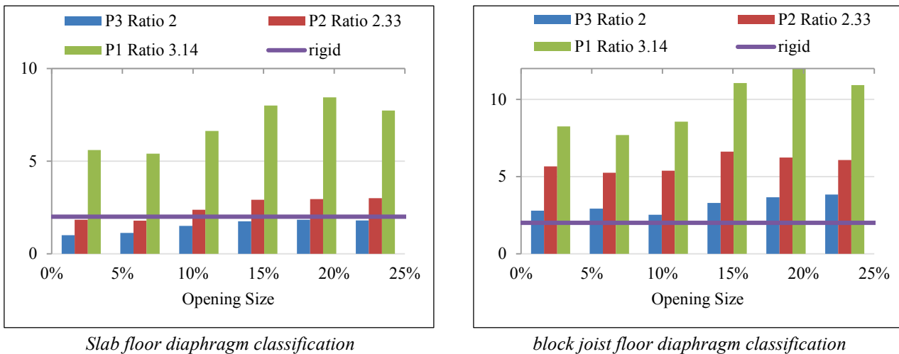
Figure 4- Diaphragm Classifications According to ASCE.
