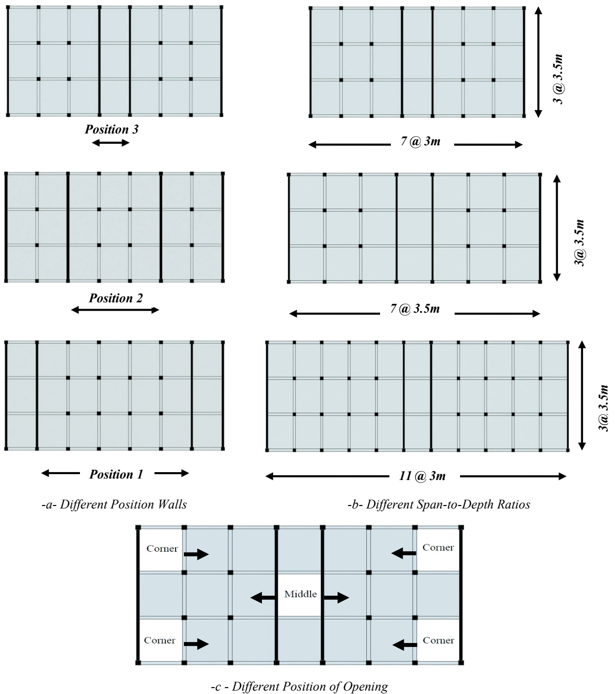
Figure 2- Building Parameters used in Analysis.
