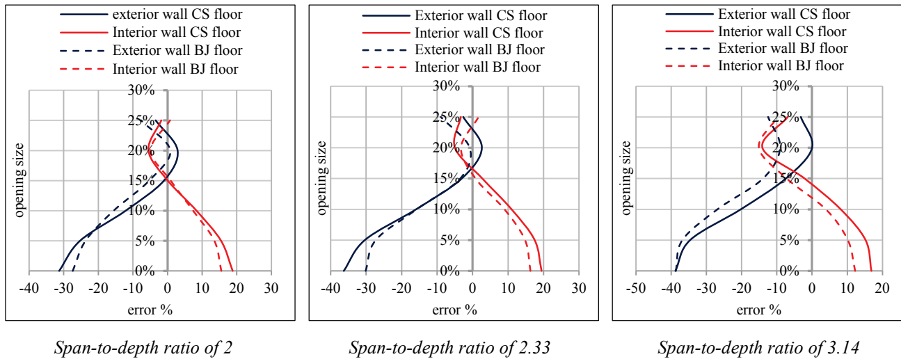
Figure 8- Error between finite elements analyzes and inertia method for position 3
