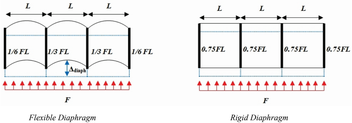
Figure 5- Distribution of Horizontal Forces in the Wall.
