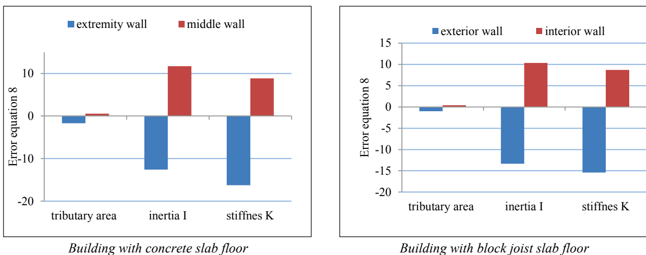
Figure 9- Distribution shear force in walls for building of 3.14:1 aspect ratio assumed rigid and with opening of size 0.64%
