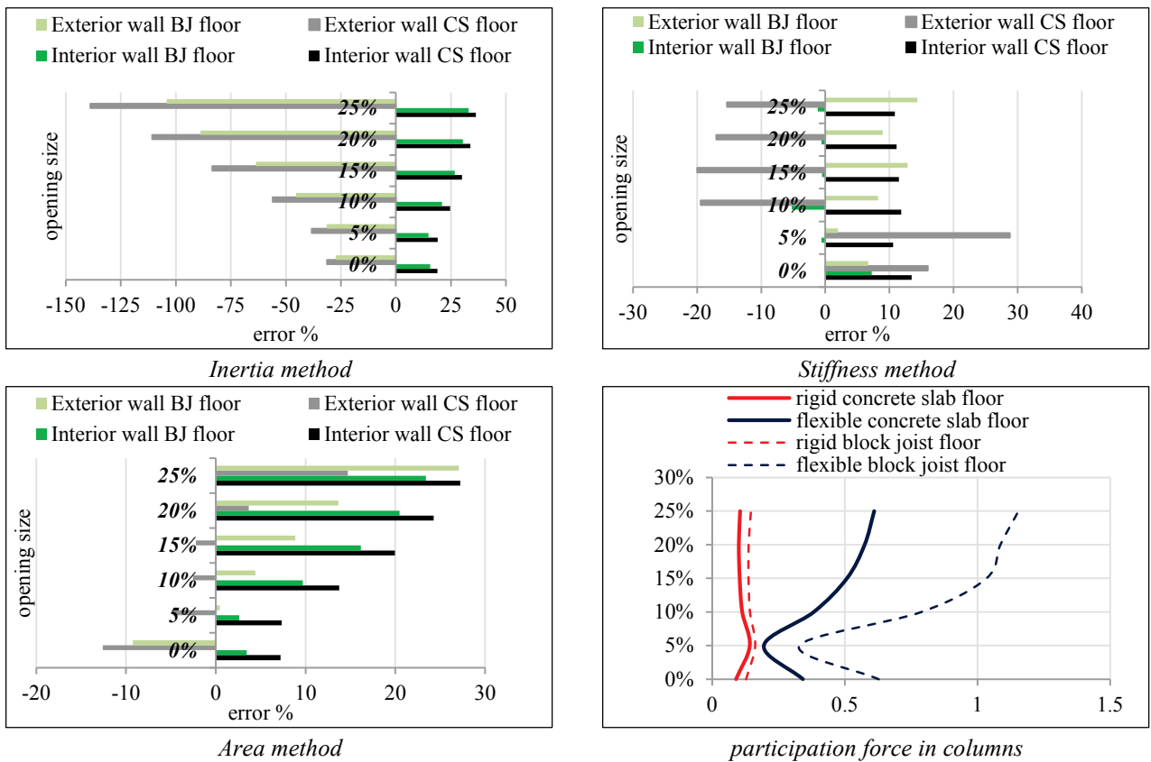
Figure 7- Error of distribution horizontal forces in shear wall for position 3 ratio 2:1 flexible diaphragms (opening located in corner)
