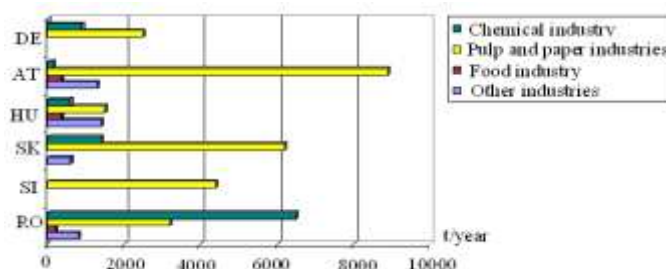
Figure 2 Direct emissions of total organic carbon per relevant types of industries in European Union Member State (2004) (from ICPDR 2009a)
