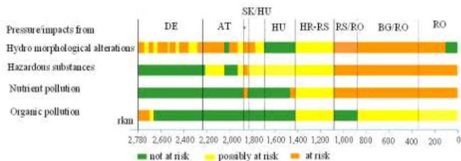
Figure 10 Results of the risk analysis for the entire Danube River length (2004) (from ICPDR 2009a )
