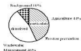
Figure 6 Sources of the P emissions 1998-2000 into the river system of the Danube basin (from Schreiber H. et al. 2003)
