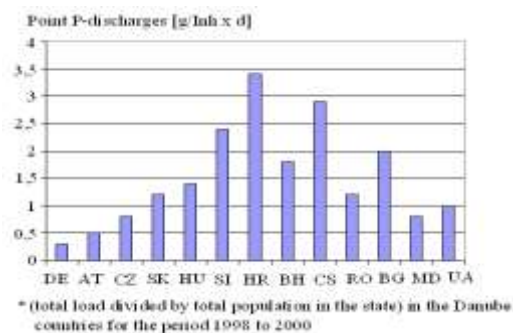
Figure 4 Inhabitant-specific P discharges from point sources* (from ICPDR 2005c)
