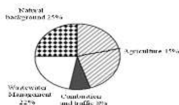
Figure 5 Sources of N emissions 1998-2000 into the river system of the Danube basin (from Schreiber H. et al. 2003)
