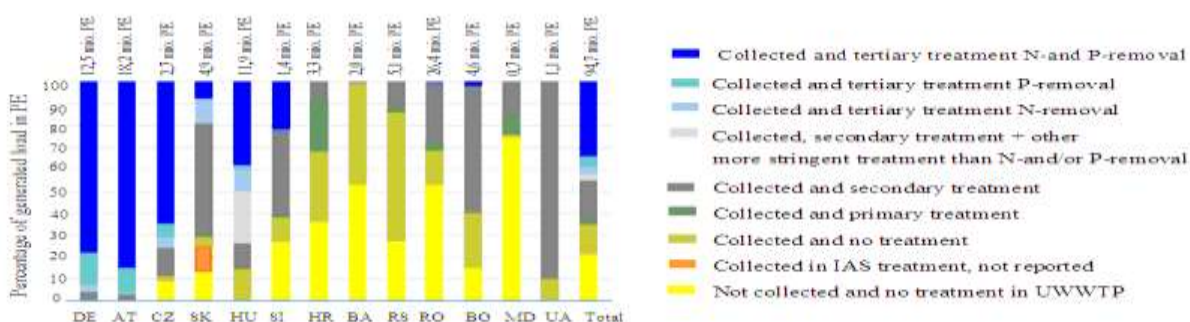
Figure 1 Wastewater treatment of the generated load from agglomerations \geq 2,000 PE (population equivalent)-reference year 2005/2006 (existing wastewater treatment plants; existing treatment levels and degree of connection to wastewater treatment throughout the entire DRB by country) (from ICPDR 2009a)
