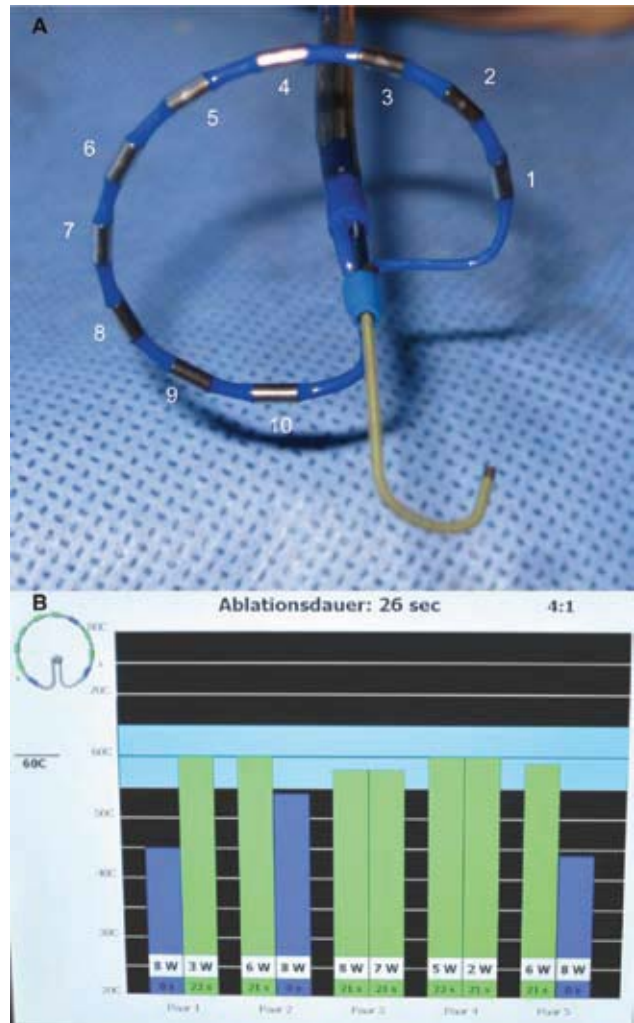
FIGURE 1. PVAC™ (A) and monitor view of the GENius™ generator (B). A - The PVAC™ catheter is an eccentric over-the-wire catheter with 10 platinum electrodes mounted on a nitinol frame. B - The GENius™ generator displays measured temperatures and indicates applied energy in bars for each PVAC electrode. Green bars indicate electrodes achieving the target temperature zone (55 to 65 °C).
