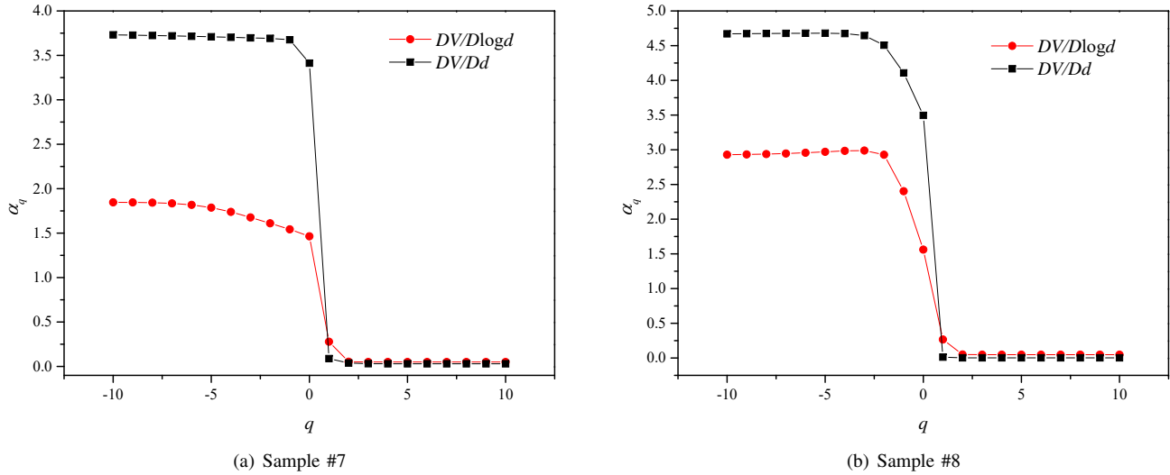
Fig. 11. The correlations between the \alpha_q and q .
