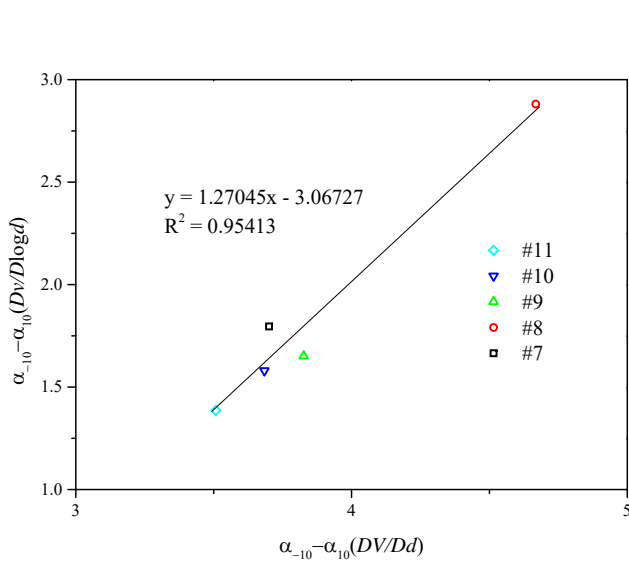
Fig. 12. Relationship between heterogeneity index of pore size distribution data from two different presentations (Sample #7 to Sample #11).
