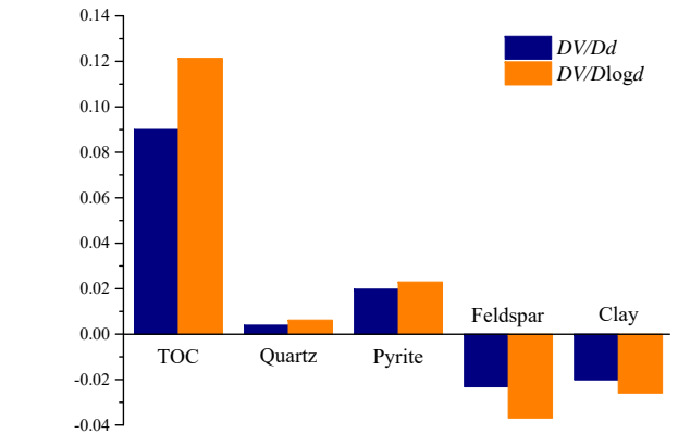
Fig. 13. The influence of individual minerals/TOC on the heterogeneity from the pore size distribution data from the two different presentations.
