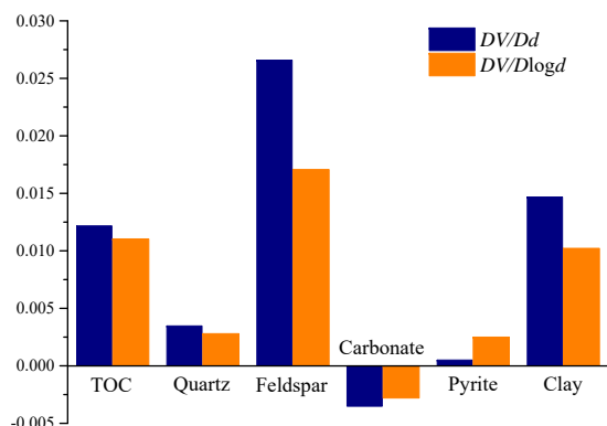
Fig. 8. The Influence of the minerals/TOC on the heterogeneity of pore size distributions on the two different presentations of the data.
