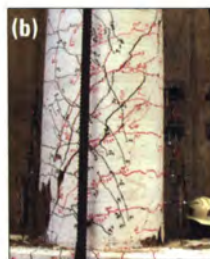
Above: Large-scale structural testing in UMR's Structural Engineering Laboratory to simulate the effect of a strong earthquake. (a) Experimental setup. (b) Damage under earthquake loads.
