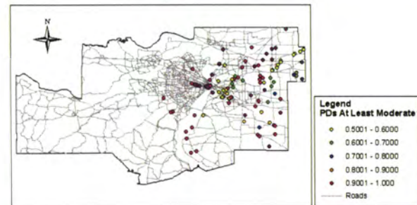
Above: Bridges in St. Louis with 50 percent probability of damage (PD) due to a Mw 7.0 scenario earthquake event in Germantown, St. Louis.
