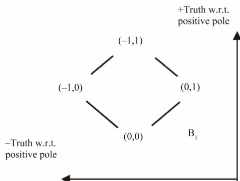
Figure 2. Hasse diagrams of B_1 in YinYang bipolar geometry.
