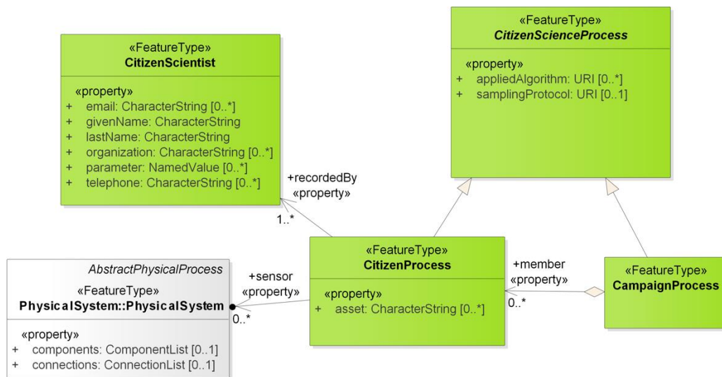
Figure 2: CitizenScienceProcess Model
