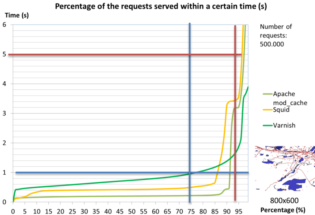
Figure 12: Comparison of Software for 800x600 px PNG
