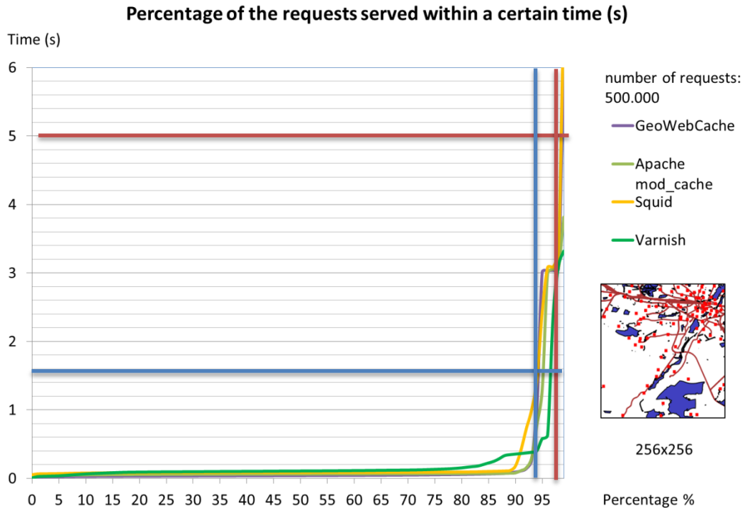
Figure 11: Comparison of Software for 256x256 px PNG
