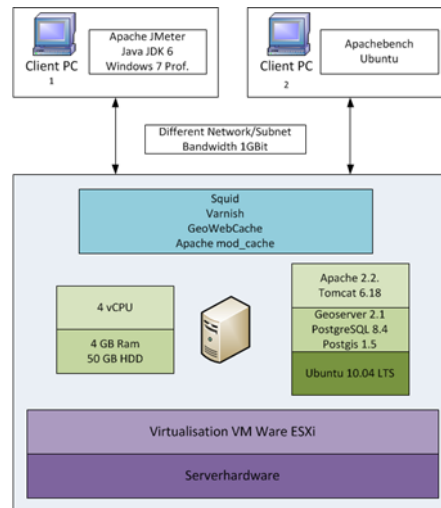
Figure 10: Testbed with Test Arrangement
