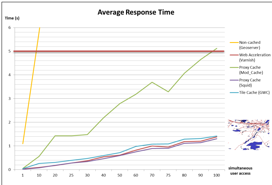
Figure 13: Response Time for the Grouplayer
