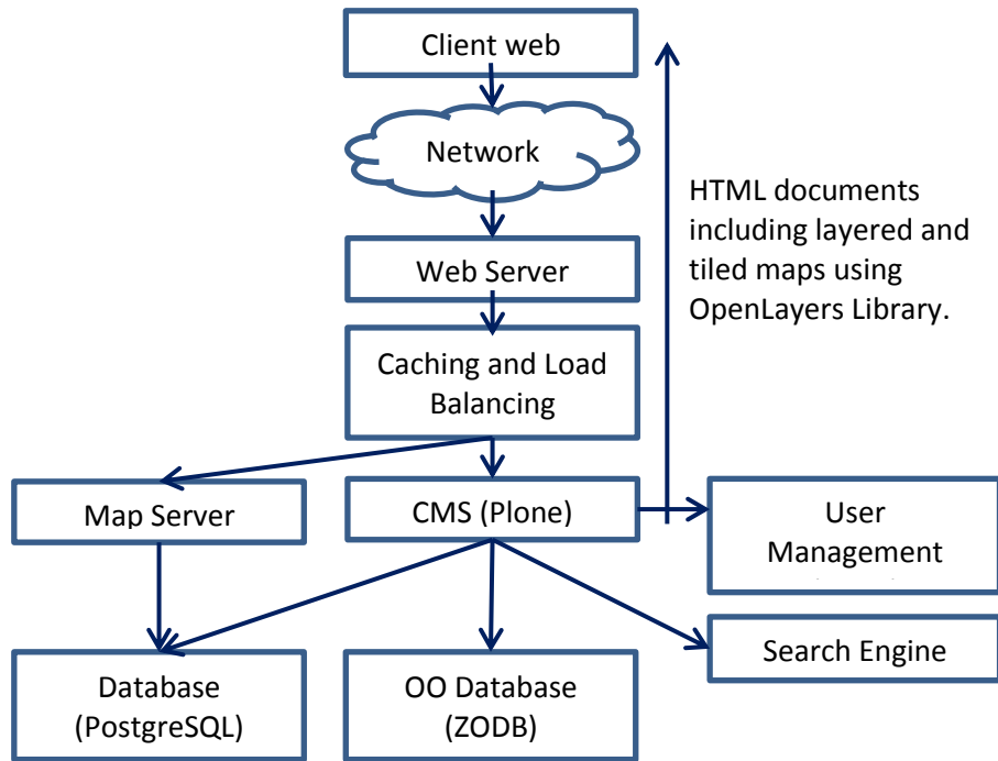
Figure 3: Component Architecture of the Implemented C2 System
