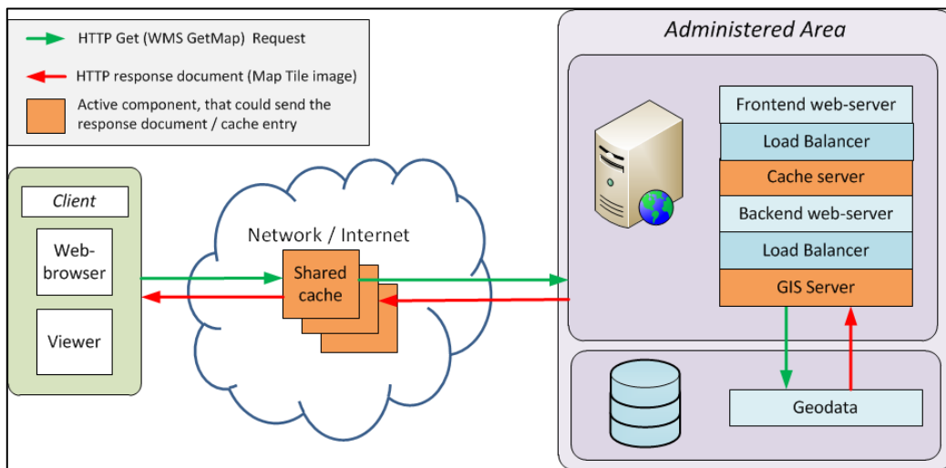
Figure 7: Schema of WMS GetMap Request - Response Communication Path and Managing Areas
