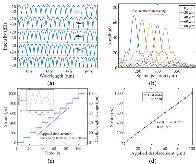
Figure 4. The calibration result of the strain sensor. (a) The recorded interference spectra for five different displacement measurements: 0 \mu\text{m} , 20 \mu\text{m} , 40 \mu\text{m} , 60 \mu\text{m} and 80 \mu\text{m} ; (b) Spatial spectra of the sensor at five different displacement measurements; (c) Cavity length change and strain with respect to applied displacement. In the experiment, the displacement applied to the right limit disc was increased from 0 to 100 \mu\text{m} with a step of 10 \mu\text{m} . In each step, 10 measurement points were recorded. The inset plots the strain under a displacement setting of 60 \mu\text{m} in a time period of 10 s; (d) The measured relationship between the strain and applied displacement. A curve fit was applied to the test data. R-square equals to 1, revealing a perfect linear relationship.
