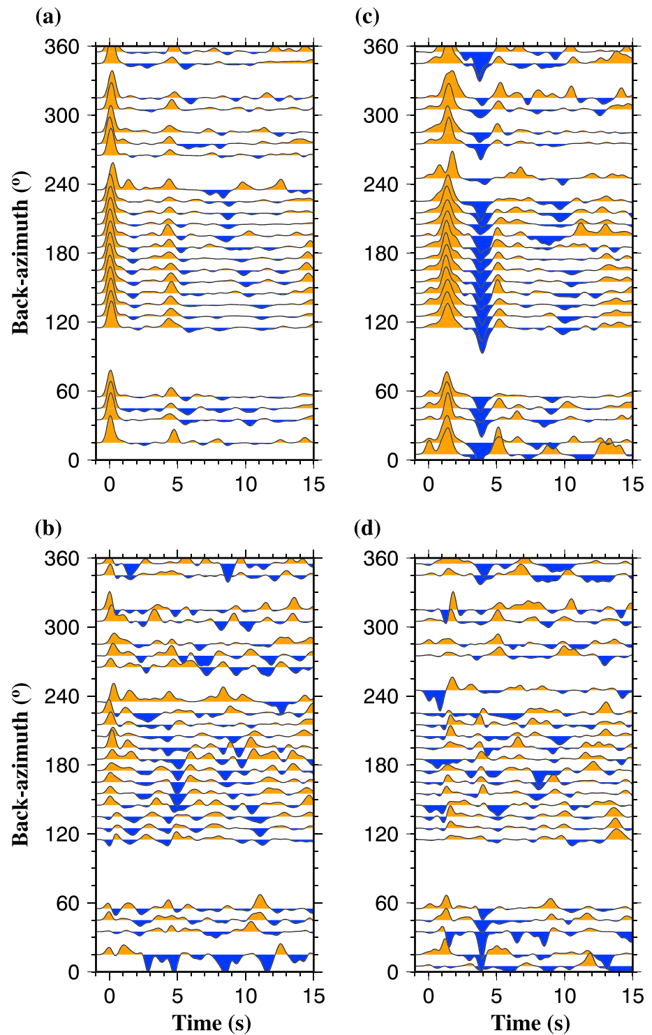
Figure 3. Example RFs plotted against the BAZ. (a) Radial RFs recorded by station A207 (40.58°N, 117.01°E; see Figure 1) situated on bedrock. (b) Transverse RFs recorded by station A207. (c) Radial RFs recorded by basin station A010 (37.86°N, 116.30°E; see Figure 1) located in a sedimentary basin. Note that in (c), the small arrival at time zero is the direct P wave, while the largest arrival is the P to S conversion from the bottom of the sedimentary layer. (d) Transverse RFs recorded by station A010. RF = receiver function.
