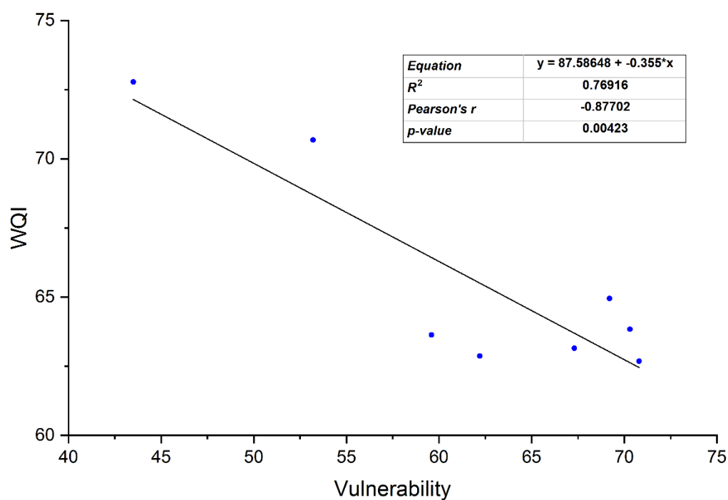
Figure 8. Comparison showing the relationship between watershed vulnerability and WQI.
