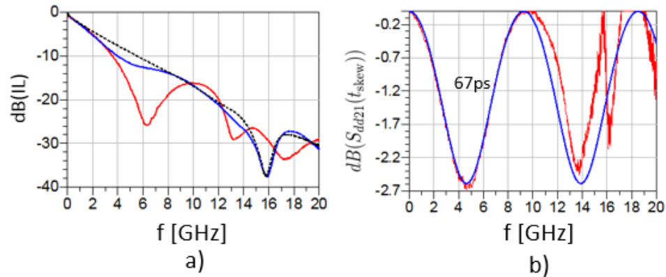
Figure 9. a) Red line shows measured single-ended IL ( S_{21} ) in 15" MS with about 22% forward coupling. Dashed black and solid blue lines show differential IL with approximately 0ps and 67ps TDS, respectively. b) the additional differential IL due to TDS obtained in measurements (red line) and predictions from (4) with tuned coupling-skew factor \alpha = 0.65 found from fitting to simulations above (blue line).
