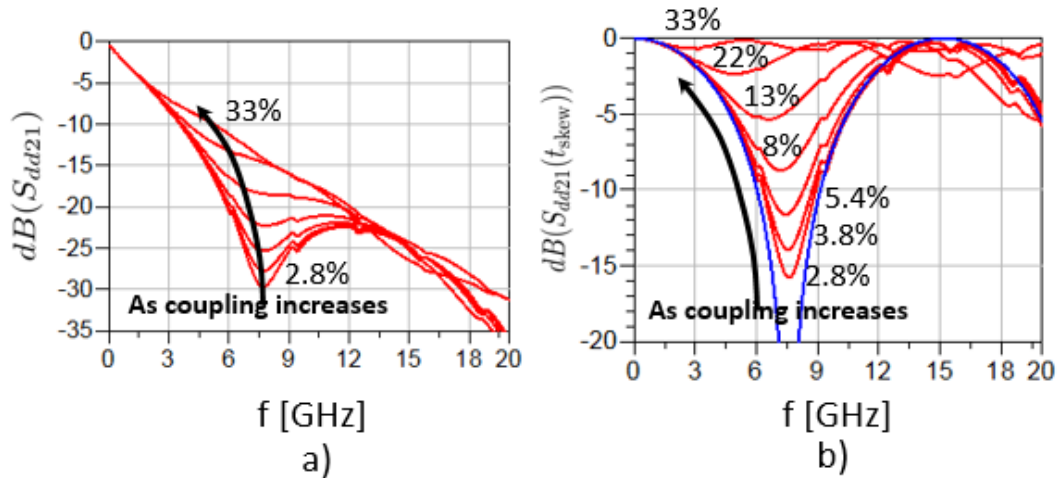
Figure 6. a) Simulated differential IL and b) additional differential IL (red lines) due to TDS in 15'' MSs with several strength of forward coupling and fixed t_{skew} = 67 ps. Solid blue line in b) shows predictions from (2) with t_{skew} = 67 ps.
