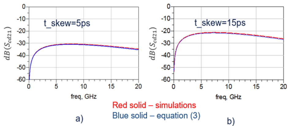
Figure 14. The to common mode conversion due to skew vs frequency.
