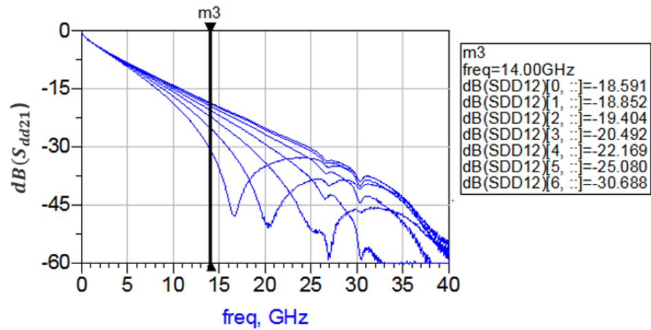
Figure 11. Measured loss vs frequency for different P/N skew introduced by different time delay cables.
