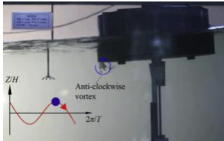
Figure 15. Vortex shedding on flat-bottom buoy [50]
