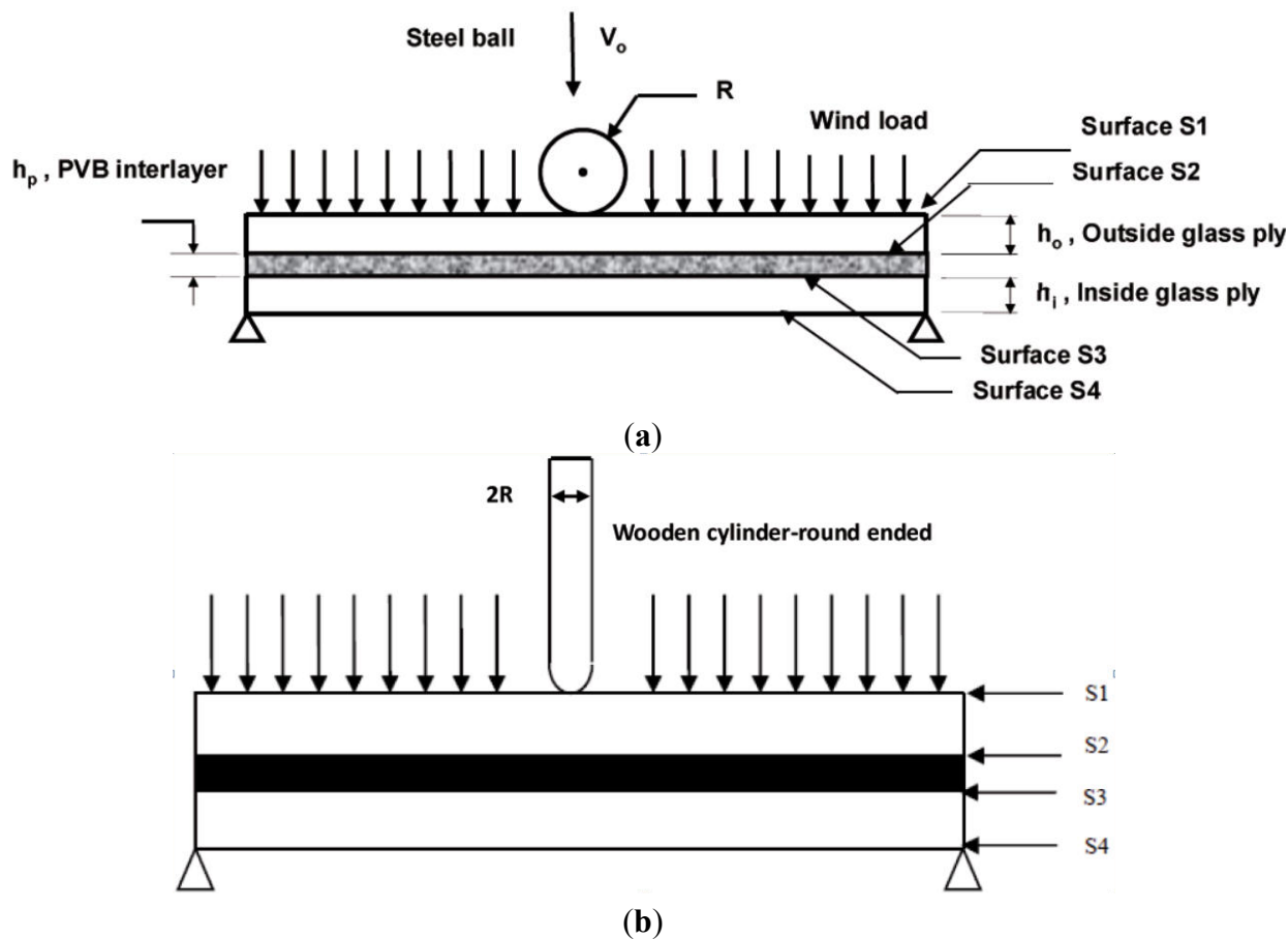
Figure 1. Schematic of different missile types impacting on 2-D laminated glazing. (a) Small missile; (b) Large missile with round impacting end; (c) Large missile with flat impacting end.
