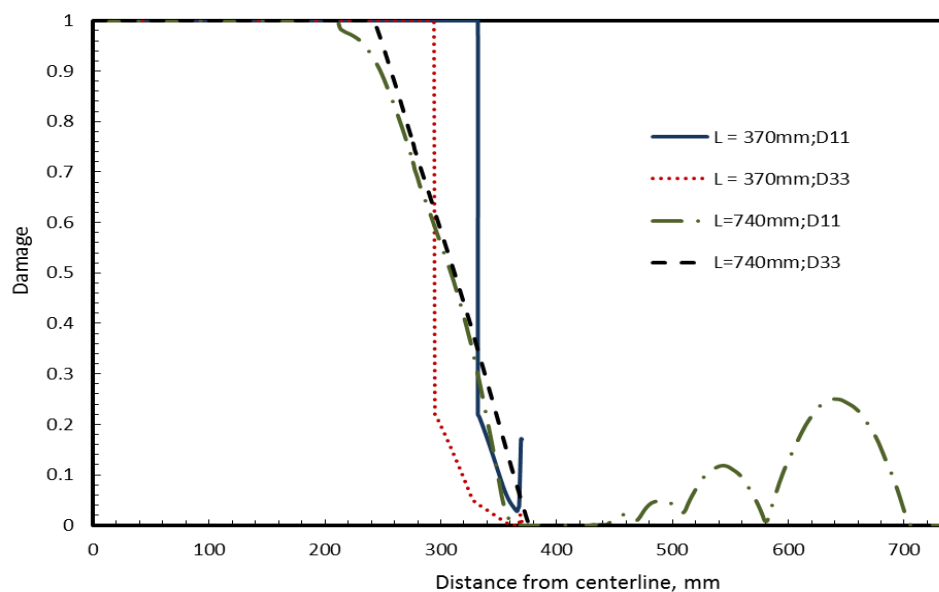
Figure 15. Effect of panel area on Damage variables D_{11} (web-shaped), D_{33} (star-shaped) at surface S4 for large missile (round end) impact.
