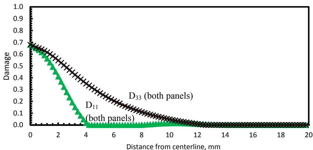
Figure 15. Effect of panel area on Damage variables D_{11} (web-shaped), D_{33} (star-shaped) at surface S4 for large missile (round end) impact.
