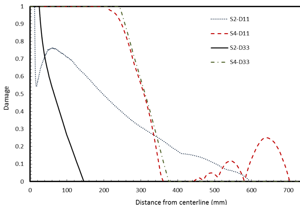
Figure 7. Damage variables D_{11} (web-shaped) and D_{33} (star-shaped) at surface S2 and surface S4 for a large missile (round end) impact.
