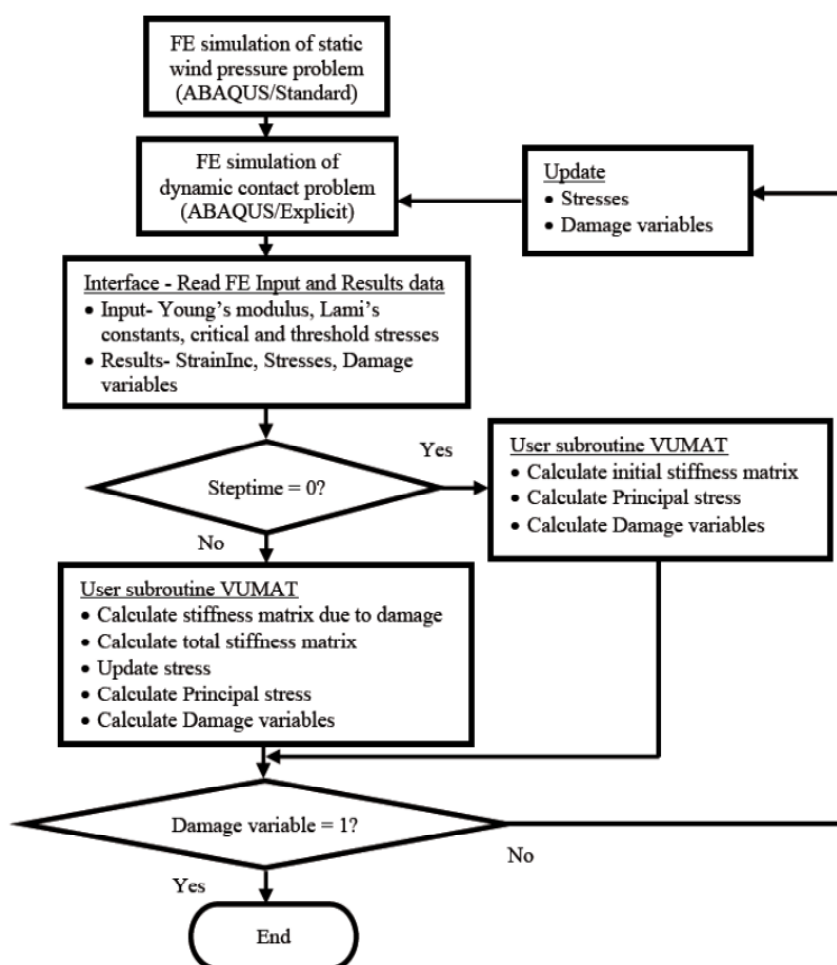
Figure 2. Flow-chart of the computational process.
