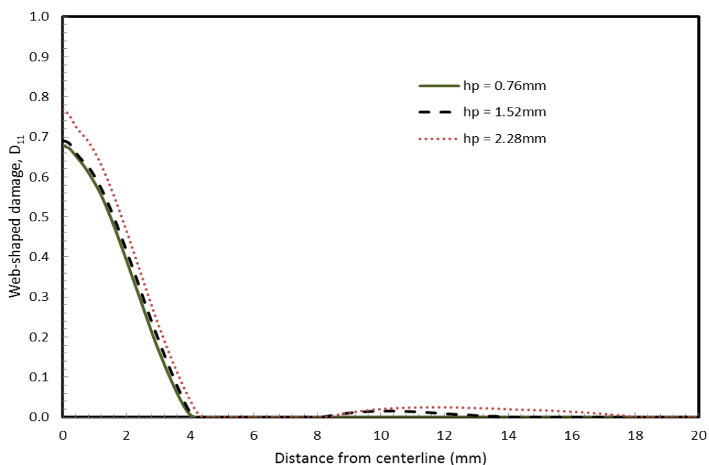
Figure 8. Effect of polyvinyl butyral (PVB) interlayer thickness on web-shaped damage, D_{11} on surface S2 for small missile impact.
