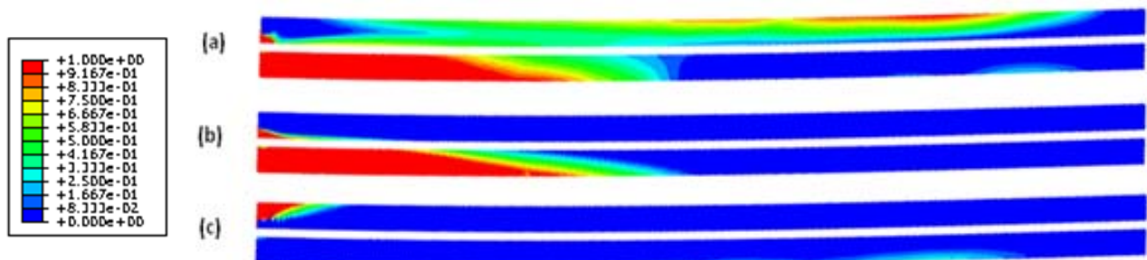
Figure 5. Contour plots of damage in laminated glass at 3.4 ms after impact for large missile with round end configuration: (a) web-shaped damage D_{11} ; (b) star-shaped damage D_{33} ; (c) shear damage D_{12} .
