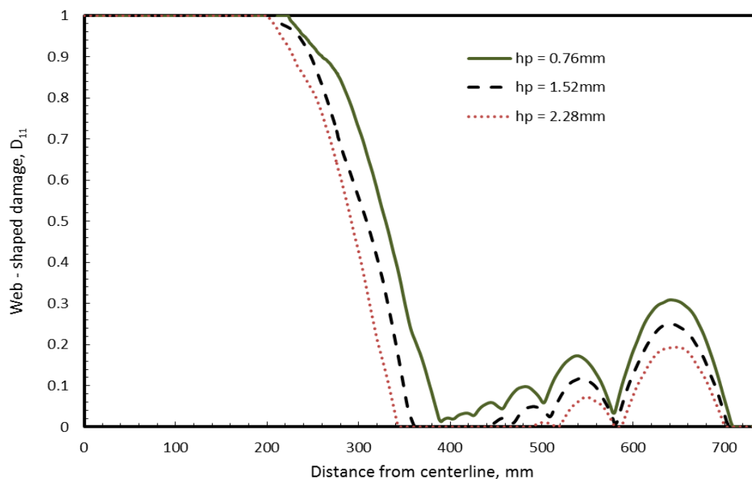
Figure 9. Effect of PVB interlayer thickness on web-shaped damage, D_{11} on surface S4 for large missile (round end) impact.
