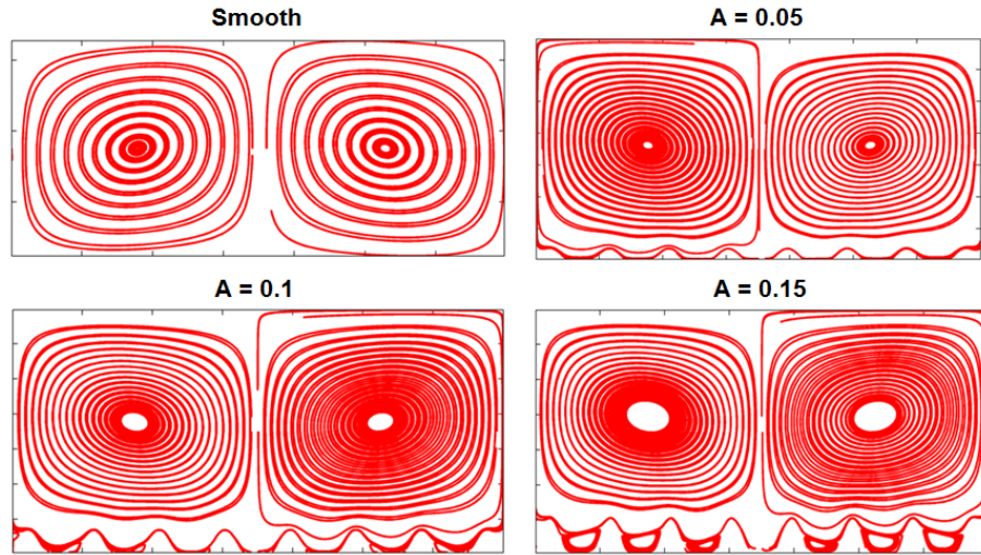
Figure 4-12: Velocity Streamlines for Different Amplitude and Constant Number of Roughness Elements of 8 at Bottom Wall for Re = 1 \times 10^4
