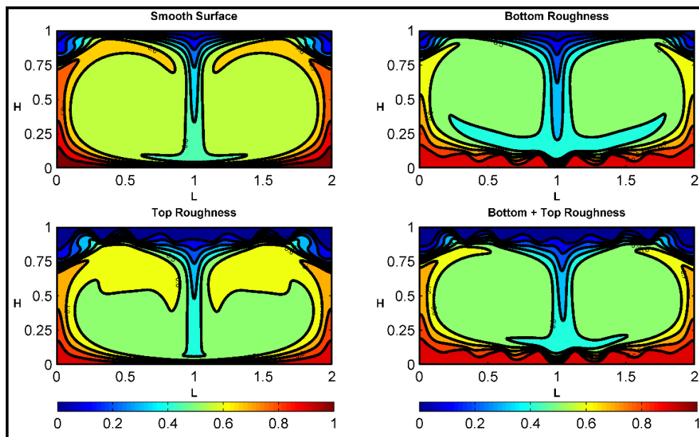
Figure 3-14: Isotherms Behavior at Ra = 10^6 amplitude 0.1 in Smooth and Rough Cavity
