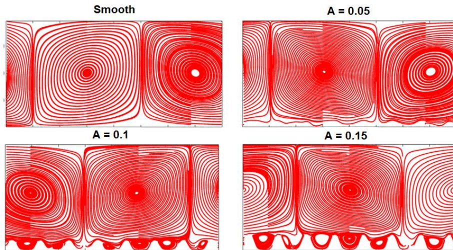
Figure 4-13: Velocity Streamlines for Different Amplitude and Constant Number of Roughness Elements of 8 at Bottom Wall for Re = 5 \times 10^5
