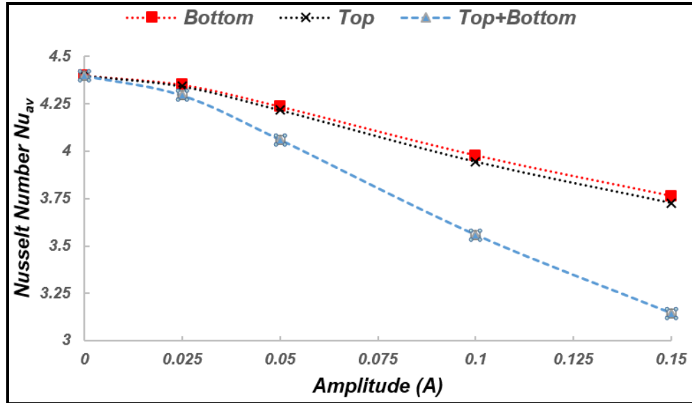
Figure 3-7: Variation of Average Nusselt Number with Roughness Amplitude for Ra = 10^5
