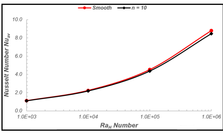
Figure 3-2: Average Nu with A - 0.025 and Varying Number of Roughness Elements
