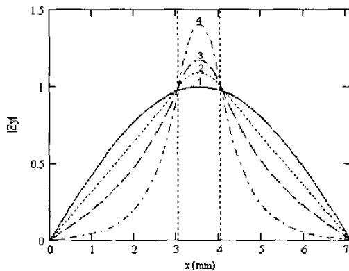
Fig 1: Electric field distribution in a rectangular waveguide loaded with a 1 mm-thick dielectric slab having various permittivities at 35 GHz.
