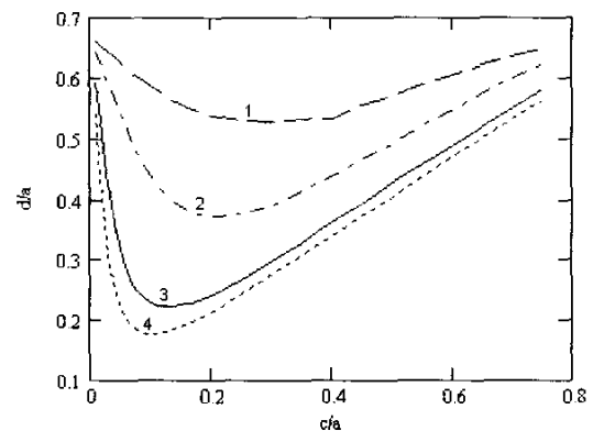
Fig 3: The extent of normalized effective electric field localization, d/a , vs. normalized slab width ( c/a ) for different dielectric permittivity of the slab.
