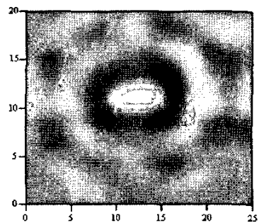
Fig 5: Image of a pitting with a diameter of ~1 mm and a depth of ~1 mm using a dielectric slab-loaded rectangular waveguide at Ka-band.
