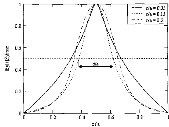
Fig 2: Normalized electric field intensity distribution in a rectangular waveguide loaded with a dielectric slab with permittivity of \epsilon'_r = 9.8 for different normalized slab width c/a .
