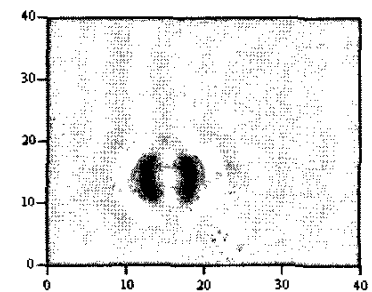
Fig 7: Image of a pitting with a diameter of ~1 mm and a depth of ~1 mm using a single tapered waveguide at Ka-band.
