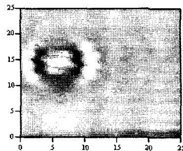
Fig 6: Image of a pitting with a diameter of ~1 mm and a depth of ~1 mm using a double tapered waveguide at Ka-band.
