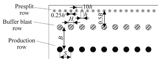
Fig. 2. Conceptual diagram of buffer blast holes used in conjunction with presplitting.
