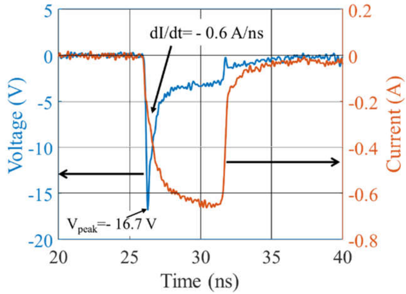
Figure A.8 Voltage and current waveform of 40 V TLP injection to the TVS sample
