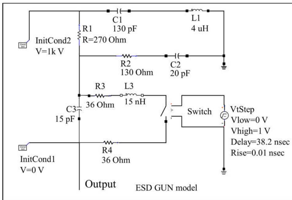
Figure 3.9. ESD gun contact discharge model
