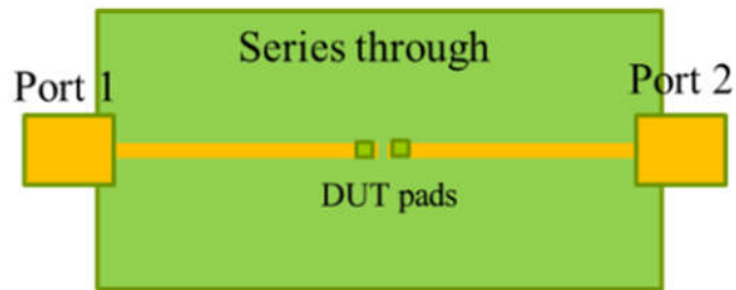
Figure A.1 Series through test fixture
