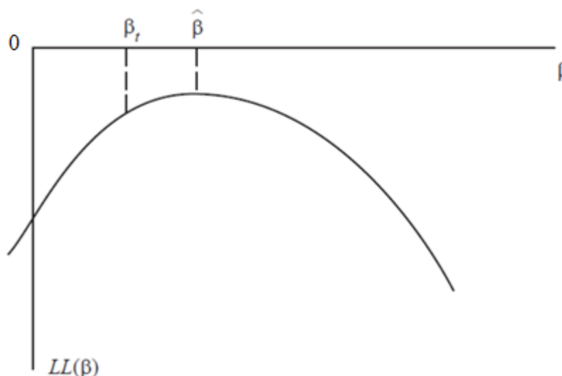
Figure 6-3. Maximum likelihood estimate (Train, 2002)
