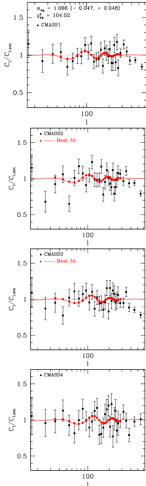
Figure 7. Best-fit result using the combinations of CMASS1, CMASS2, CMASS3, and CMASS4 and using AOB1. We derive \alpha - 1 = 6.609^{+4.82}_{-4.68}\% , i.e., 4% deviation from the fiducial value based on WMAP7. The black data points in the four panels with error bars show the measured C_\ell divided by a smooth fit at CMASS1, CMASS2, CMASS3, and CMASS4. The red lines show the resulting best-fit C_\ell and the red circles show the best-fit band power C_\ell after the window function effect is considered.
