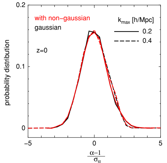
Figure 8. Distribution of the shift parameter \alpha for k_{\text{max}} = 0.2 (solid curves) and 0.4 h \text{ Mpc}^{-1} (dashed curves), respectively. The horizontal axis \alpha - 1 is divided by the 1\sigma error computed from the Fisher matrix. The red and black curves are the results with and without the non-Gaussian errors, respectively. The distribution of \alpha is well described by a Gaussian distribution with the width of the 1\sigma Fisher error.
