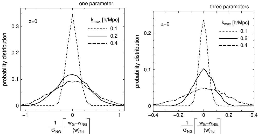
Figure 5. As in the previous figure, but for the distribution of the differences between the best-fit values of w computed from Equation (8) with and without non-Gaussian errors. The \sigma_{\text{NG}} is the 1\sigma error computed from the Fisher matrix with the non-Gaussian errors.
