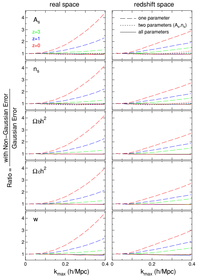
Figure 3. Ratio of the marginalized errors with and without the non-Gaussian errors, as a function of k_{\max} . The solid curves show the results for our fiducial set of five cosmological parameters as shown in each panel. For comparison the dashed curves show the results for the unmarginalized errors or equivalently for the case of one-parameter fitting in each panel. Also, in the panels for A_s and n_s the dotted curves show the results for the two-parameter fitting of (A_s, n_s) , which appear to be between the solid and dashed curves. It is clear that the non-Gaussian errors degrade the unmarginalized errors by up to a factor of five. (A color version of this figure is available in the online journal.)
