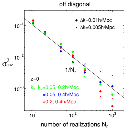
Figure 10. Dispersions among the power spectrum covariances each of which is estimated from the N_r realizations (a subset of the while 5000 realizations) as a function of N_r . In the vertical axis, the dispersion is defined in Equation (A7). The panel shows the result for the off-diagonal parts for varying the wavenumber bins and the bin widths. The color symbols are the simulation results, while the solid curves denote the theoretical prediction for the Gaussian density fluctuation. The plots explicitly show that the power spectrum covariances are estimated at a sub-percent level accuracy by using our whole 5000 realizations.
