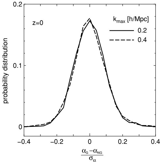
Figure 9. Distribution of the differences between the best-fit values of \alpha with or without including the non-Gaussian covariance. The solid (dashed) curve is for k_{\max} = 0.2(0.4) h \text{ Mpc}^{-1} .
