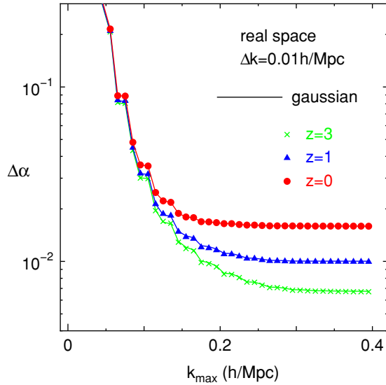
Figure 7. 1\sigma error on the BAO peak position parameterized by the stretch parameter \alpha (see the text for the definition). The symbols are the results computed from simulations, while the solid curves, which are almost on top of the symbols, show the errors computed assuming Gaussian errors.
