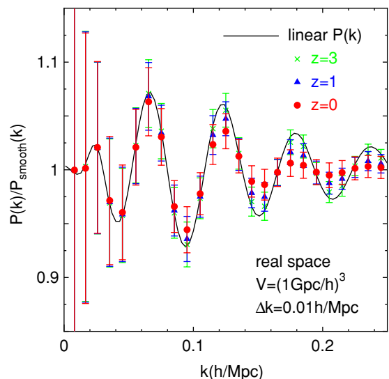
Figure 6. Real-space power spectrum divided by the smoothed spectrum for z = 0, 1 , and 3 , respectively. The symbols denote the mean of the power spectra among 5000 realizations of (1 h \text{ Gpc}^{-1})^3 volume, while the error bars denote the 1\sigma scatters. The solid curve is for the linear P(k) . The BAO features are more erased at higher k and at lower redshifts due to stronger nonlinearities.
