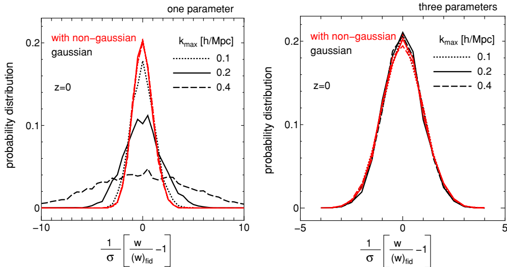
Figure 4. Distribution of the best-fit parameter w estimated for the power spectra of 5000 realizations in real space. The red (black) curve shows the result obtained with (without) the non-Gaussian error covariance in Equation (8). The dotted, solid, and dashed curves are for k_{\max} = 0.1, 0.2, and 0.4 h \text{ Mpc}^{-1} , respectively. The left panel shows the best-fit values of w for one-parameter fitting ( w alone), while the right panel shows the results for three-parameter fitting ( w, A_s, n_s ). The horizontal axis is defined as (w/w_{\text{fid}} - 1)/\sigma , where \sigma denotes the 1\sigma confidence regions computed from the Fisher matrix with and without the non-Gaussian errors for the red and black curves, respectively.
