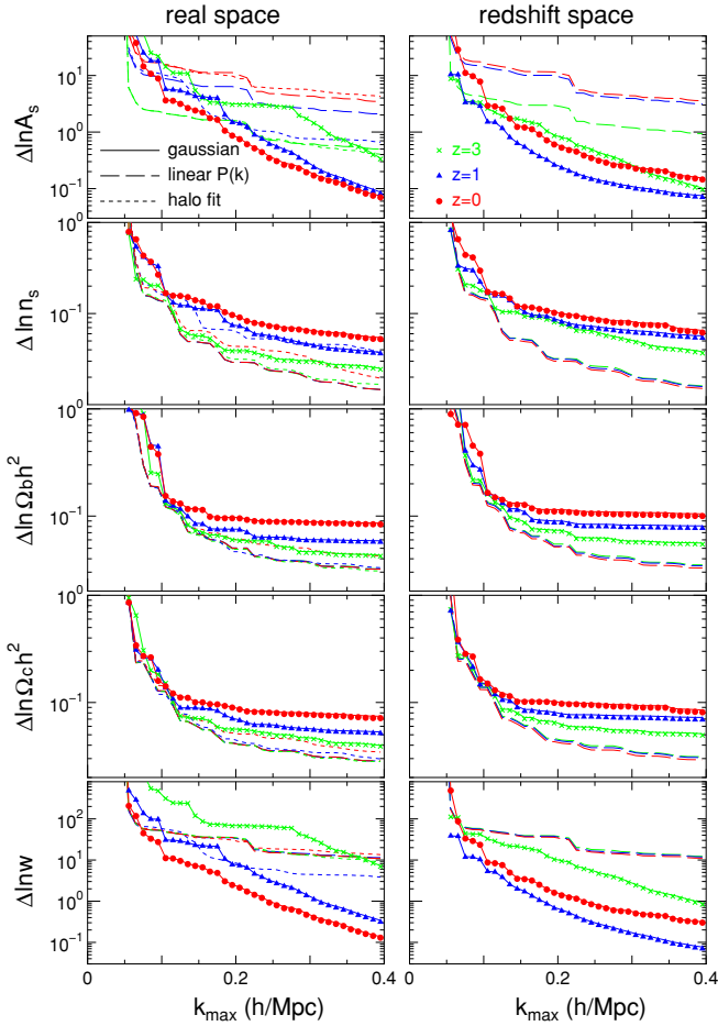
Figure 2. Marginalized errors of each parameter when including the power spectrum information up to the maximum wavenumber k_{\max} in the horizontal axis. The left and right panels show the results for the real space and redshift space, respectively. The symbols in each panel are as for the previous figure. The solid curves which lie almost on top of the symbols show the results obtained only by including the Gaussian errors in the Fisher analysis. The agreement indicates that the Gaussian error assumption is a good approximation for parameter estimations even at small scales (see the text for the details). The dashed and dotted curves are the analytical predictions that are derived using linear theory and halo fit for the power spectrum and Gaussian covariance, respectively.
