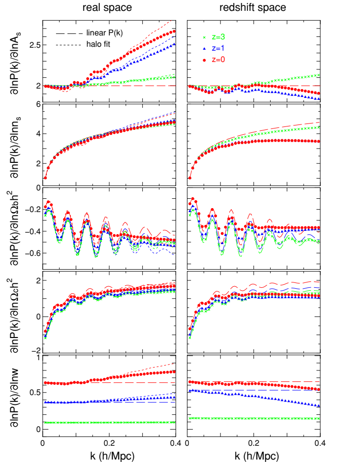
Figure 1. Derivatives of nonlinear power spectrum with respect to cosmological parameters ( A_s , n_s , \Omega_b h^2 , \Omega_c h^2 , w ) in real space (left panel) and redshift space (right). The cross, triangle, and circle symbols show the simulation results at redshifts z = 3, 1 , and 0 , respectively. The dashed curves are the linear theory predictions, the dotted curves are for the halo fit.
