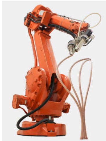
(b) Robot Deposition
