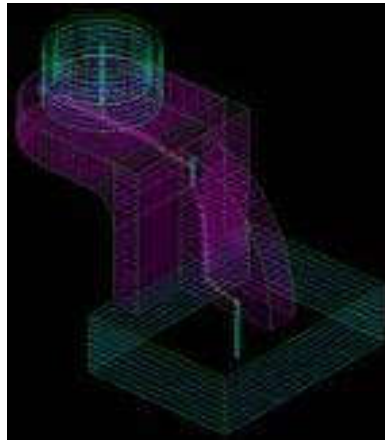
(b) Automated generated tool path for deposition and machining
