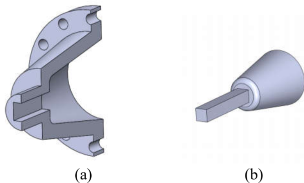
Figure 4.1 Cross section view of nozzle and the inside volume model
