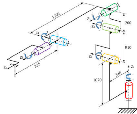
Figure 3.3 Kinematic chain schematic of Nachi Robot (SC300F-02)
