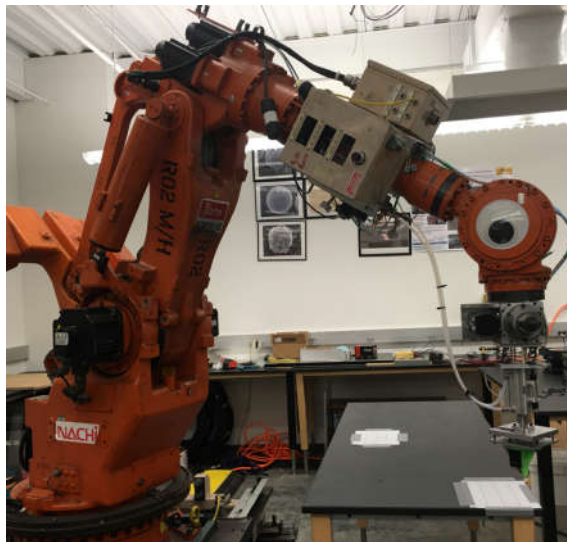
Figure 6.3 Experiments set up for accuracy evaluation of robot drawing straight line
