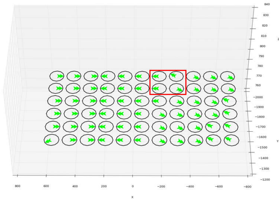
(a) X(-600,600) , Y(-1200, -1800) , Z=800
