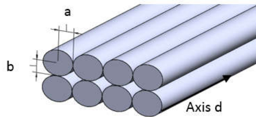
Figure 3.1 Ideal cross section of deposited filament
