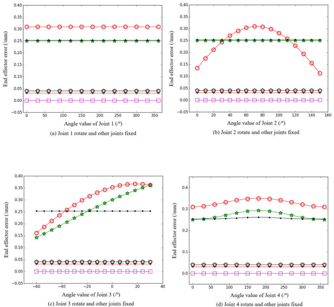
Figure 5.4 End effector error distribution when joints rotate with unified angle error
