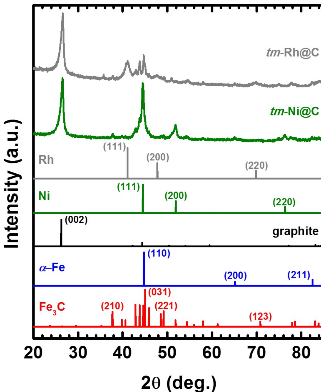
Figure S.9. Powder XRD data after transmetalation with Ni and Rh of FcPA-15 samples pyrolyzed at 1200 °C under \text{H}_2 , as shown. Both spectra are dominated by the (002) reflection of graphite and contain small amounts of \text{Fe}_3\text{C} . Owing to the overlap of the (111) reflection of Ni with the reflections from \text{Fe}_3\text{C} , reliable application of the Scherrer equation was possible only with the (111) diffraction of Rh, whose crystallite size was calculated equal to 9 \pm 1 nm.
