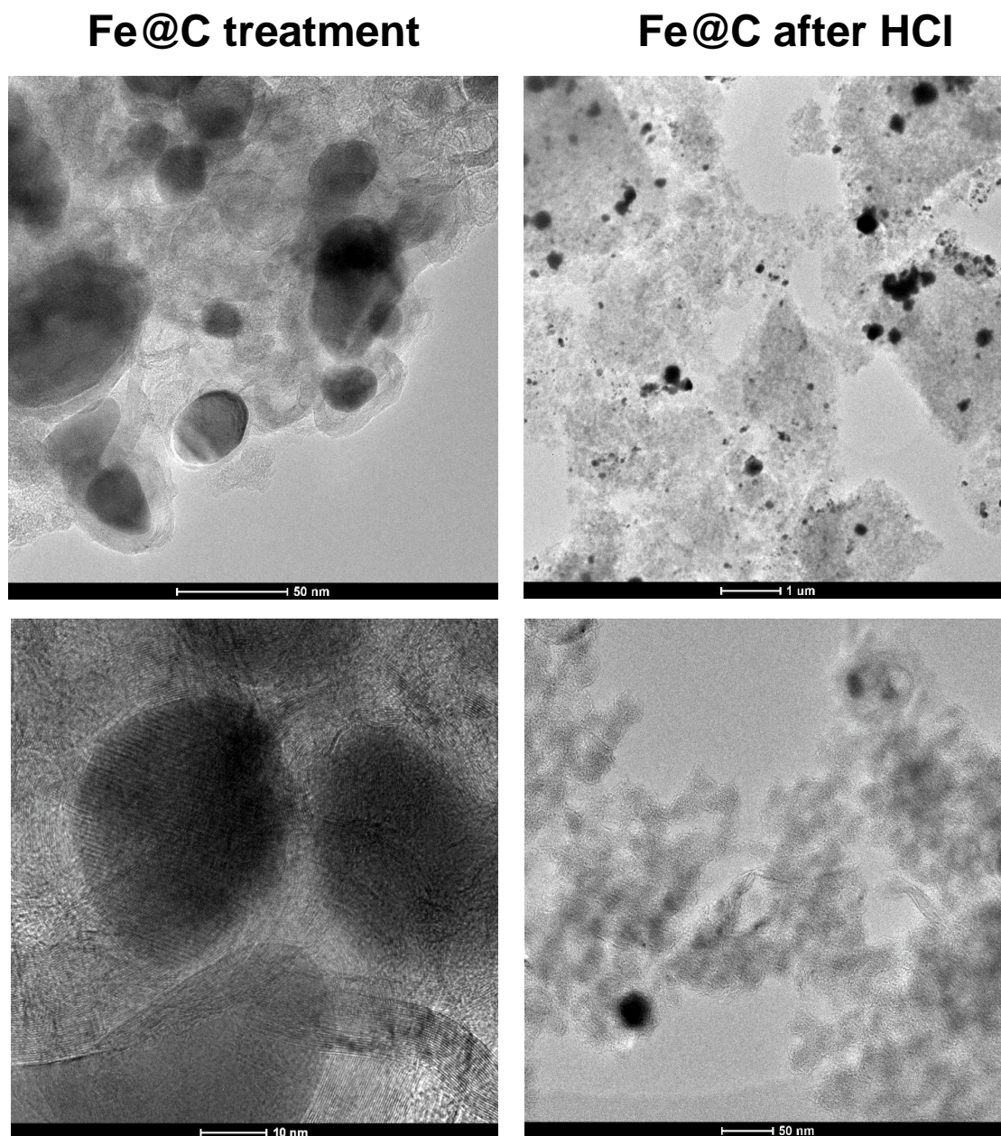
Figure S.10. TEM of samples as shown. Left: Fe@C. Left column top: Occasionally, ribbons swirl around and form pockets like those shrouding Fe(0) particles. Left Column bottom: Always Fe(0) particles are encased in ribbons. Right: Fe@C after treatment with concentrated aq. HCl at two magnifications. Consider these data together with the PXRD spectra of Fe@C before and after HCl treatment, shown in Figure S.8. (Continued on the next page.)
