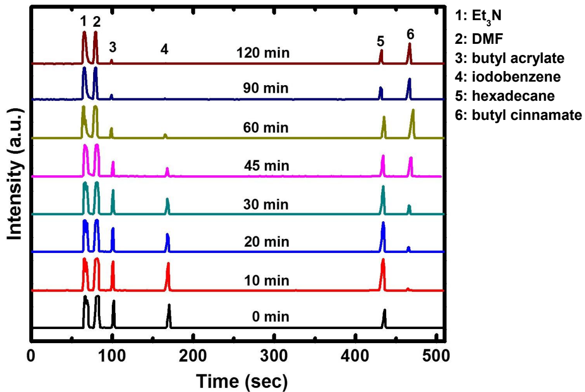
Figure S.18. GC analysis of aliquots taken out during the 1st Cycle of the Heck coupling of iodobenzene and butyl acrylate towards butyl cinnamate using a tm -Pd@C monolith as a catalyst. Results are plotted in Figure S.19.
