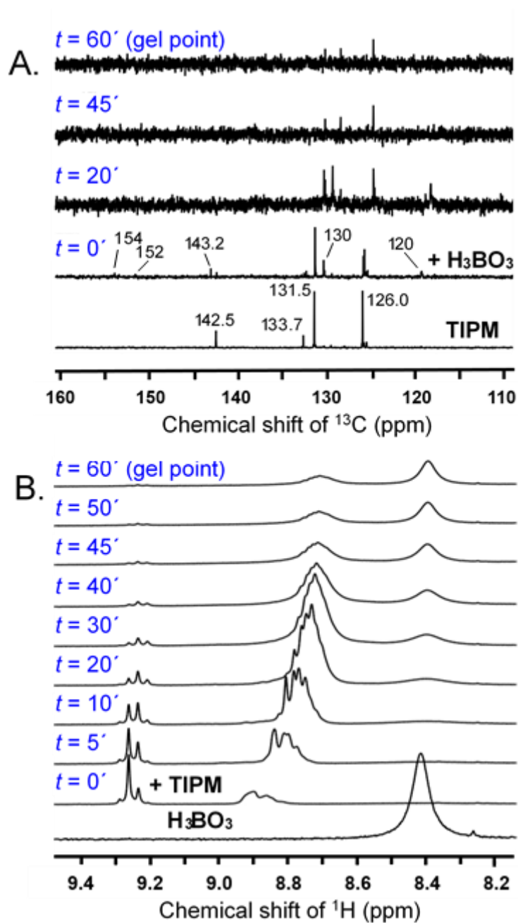
Figure 6. A. Liquid-phase ^{13}C NMR of a BPUA-4 sol in DMF- d_7 during gelation. B. ^1H NMR of a similar sol during gelation.
