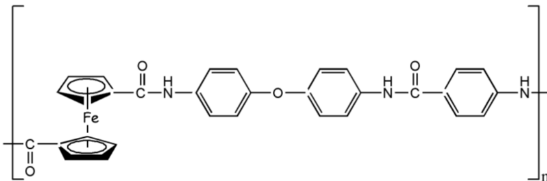
Figure 1.8. Ferrocene-incorporating polyamides synthesized via solution polycondensation.
