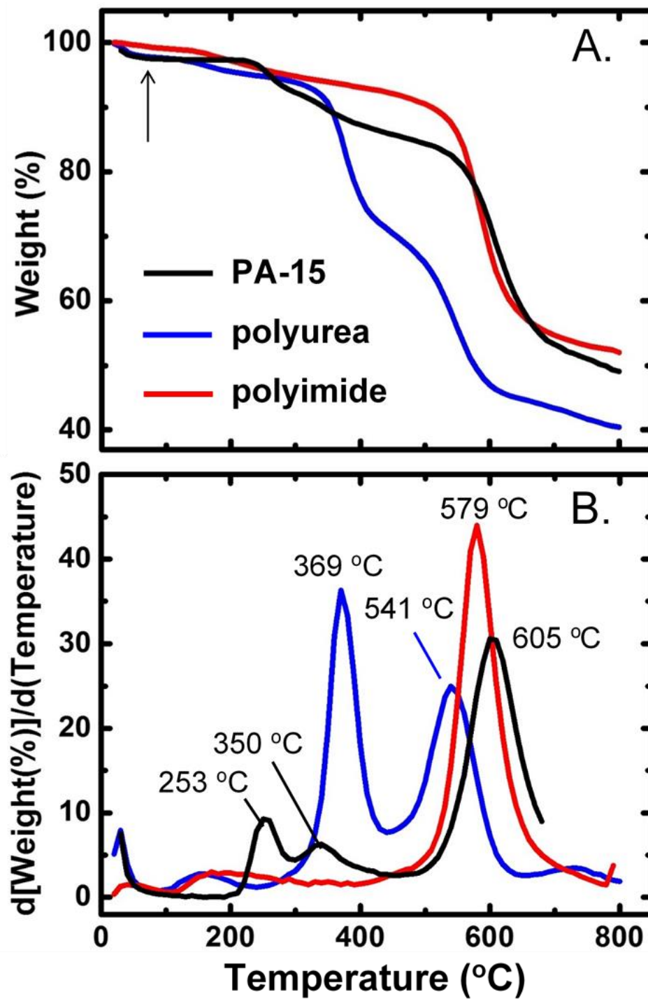
Figure 5. A. Representative thermogravimetric analysis data (TGA) under \text{N}_2 at 5\text{ }^\circ\text{C min}^{-1} of samples as shown. (Arrow points at the early mass loss by PA-15 (about 3%), which is due to loss of \text{CO}_2 . See text and Movie S.1). B. First derivative of the traces in part A.
