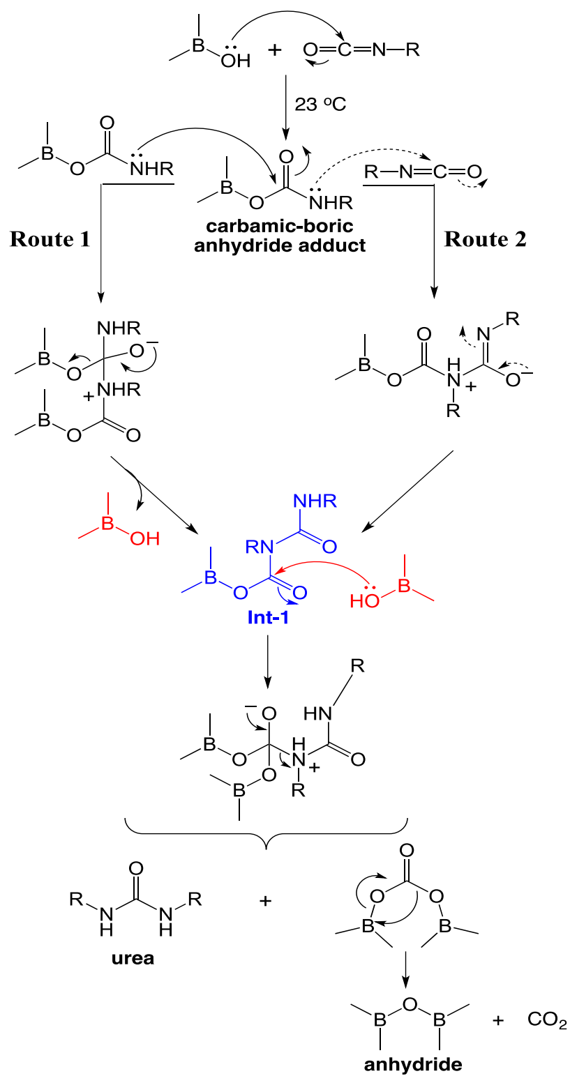
Scheme 4. Proposed mechanism for the formation of urea from an isocyanate and \text{H}_3\text{BO}_3 .
