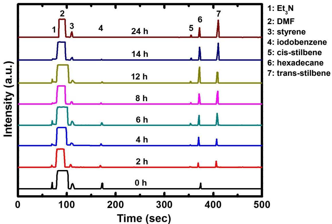
Figure S.20. GC analysis of aliquots taken out during the 1st Cycle of the Heck coupling of iodobenzene and styrene towards cis- and trans-stilbene using a tm-Pd@C monolith as a catalyst. Results are plotted in Figure S.21.
