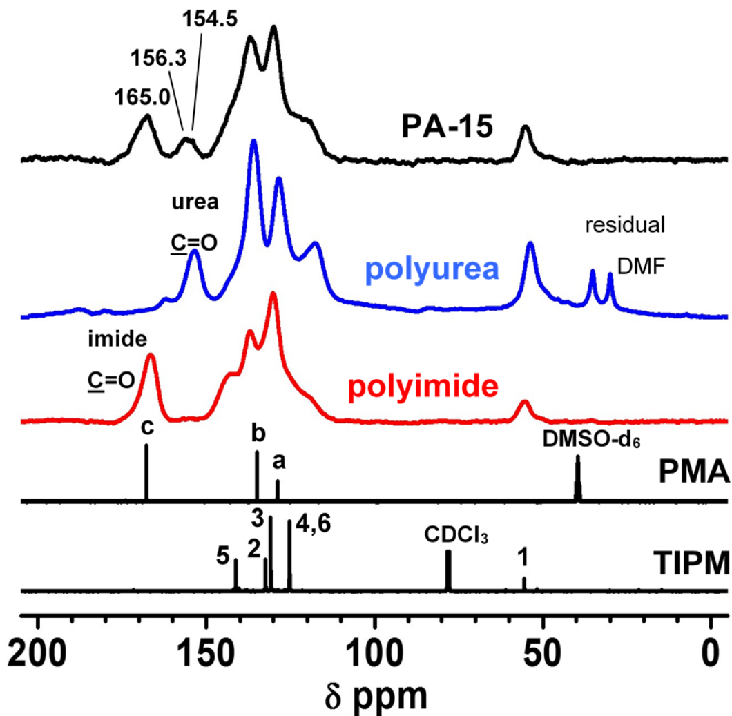
Figure 3. Top three spectra: Solid-state CPMAS ^{13}\text{C} NMR spectra of a representative PA-xx aerogel, of a TIPM/H 2 O-derived polyurea aerogel, and of a TIPM/pyromellitic anhydride-derived polyimide aerogel, as indicated. (Note, only polyurea contained residual gelation solvent: DMF.) Bottom two spectra: Liquid state ^{13}\text{C} NMR of pyromellitic acid (PMA) in DMSO-d 6 , and of TIPM in CDCl 3 . (All spectra are referenced to TMS.)
