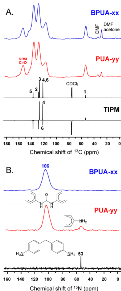
Figure 2. A Solid-state ^{13}\text{C} CPMAS NMR spectra of BPUA-xx and PUA-yy as indicated. The broad-band ^1\text{H} decoupled liquid-phase ^{13}\text{C} NMR spectrum of the monomer (TIPM) in the APT and the normal mode (bottom, and second from bottom, respectively) is included for comparison. Those spectra were obtained using 10 mg of chromium(III) trisacetylacetonate and 30 s relaxation delay. Peak assignment (refer to Scheme 3) was based on integrated intensities and the APT spectrum. (Residual gelation (DMF) and processing (acetone) solvents are marked explicitly.) B. Top two spectra: Solid-state CPMAS ^{15}\text{N} NMR spectra of BPUA-xx and PUA-yy as indicated. Structural features shown within the frame are discussed in the text. Bottom spectrum: Liquid-phase ^{15}\text{N} NMR spectrum of methylene dianiline in \text{CD}_3\text{NO}_2 .
