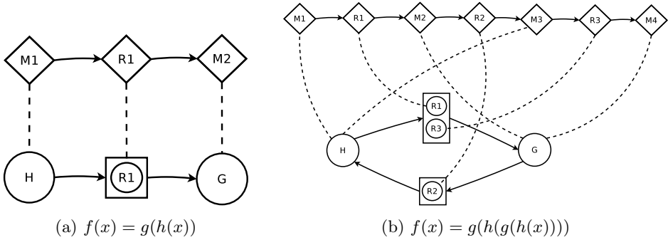
Figure 1. Examples of decompositions for Turing machines. H and G are subtasks. R_1 to R_3 are repositions. M_1 to M_4 are subDTMs.
