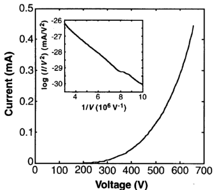
Figure 2.8. I-V curve for emission of electrons from a CNT-based electron source. Emitting area: 1mm 2 . Cathode-anode gap: 20μm. Inside: FN curve - \log(I/V^2) vs. 1/V [17].
