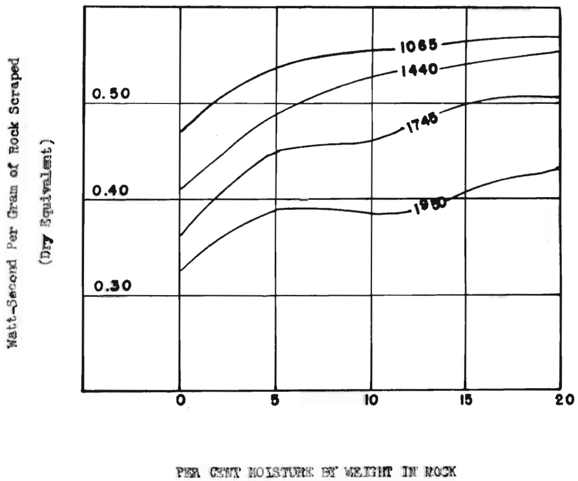
Graph 9. Relationship between moisture content and power consumption.
