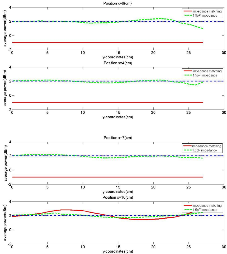
Fig 5.4: Power at reader for varying additional tag distance when tag T=30\text{cm}
