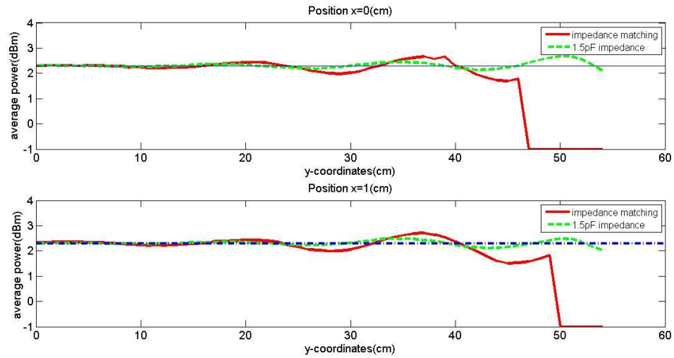
Fig 5.5: Power at reader for varying additional tag distance when tag T=60\text{cm}
