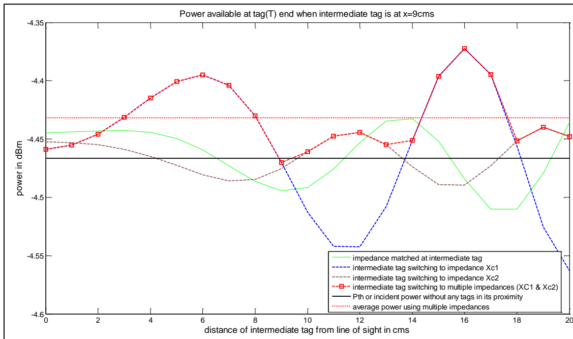
Fig 5.3: Additional tag switching to different impedances when it is at x=9cms
