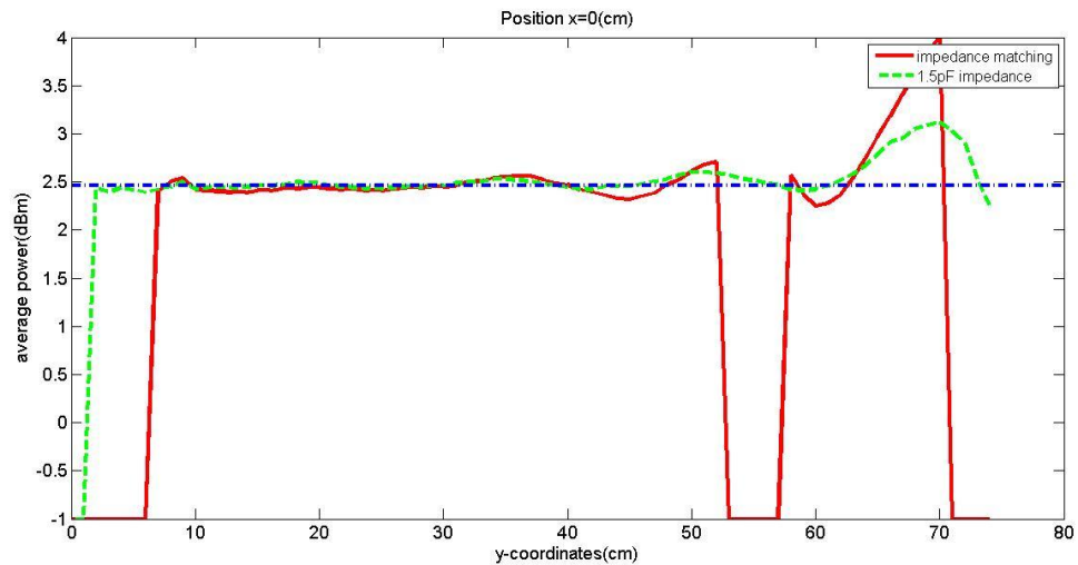
Fig 5.6: Power at reader for varying additional tag distance when tag T=80\text{cm}
