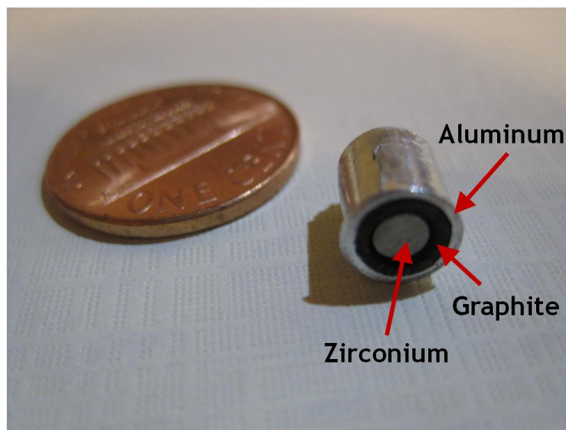
Figure 2.14. The cylindrical fuel phantom made of zirconium, graphite, and aluminum.
