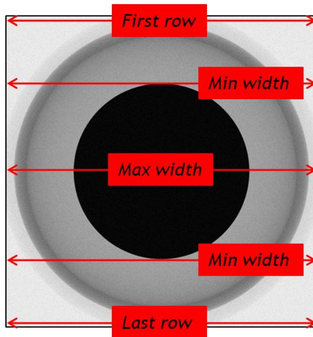
Figure 2.6. Width of a TRISO fuel kernel with respect to image row; used to calculate the centroid. This operation is performed after thresholding the image.
