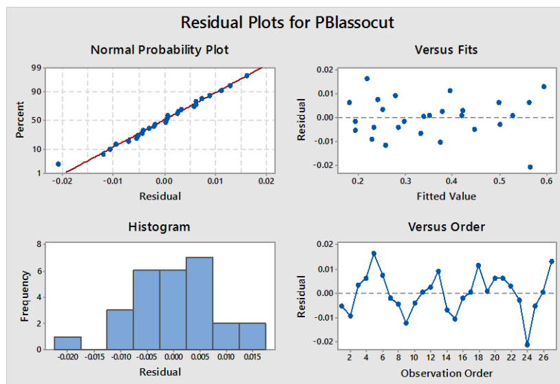
Figure 3. Residual power consumption (MQL- Blasocut)
