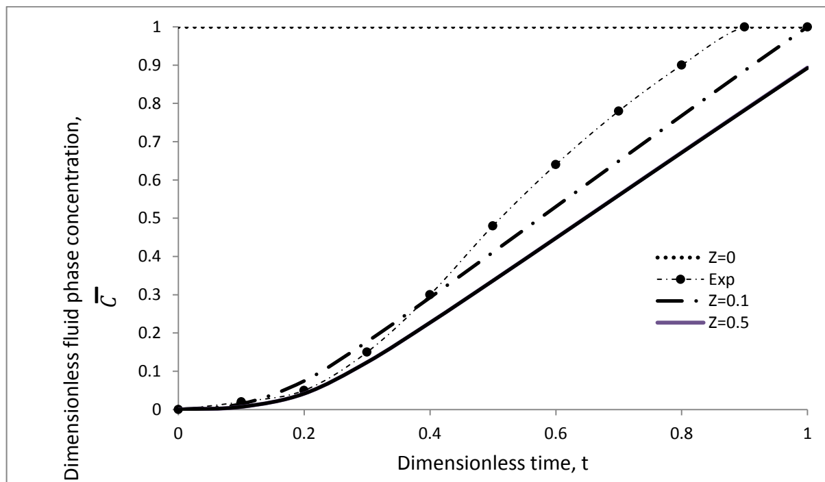
Figure 1. Plot of dimensionless fluid phase concentration of water against dimensionless time for different bed positions
