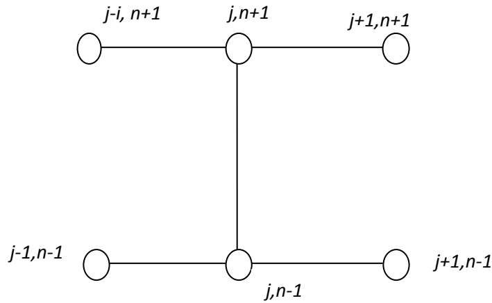
Figure 2: The Crank-Nicholson Stencil.
