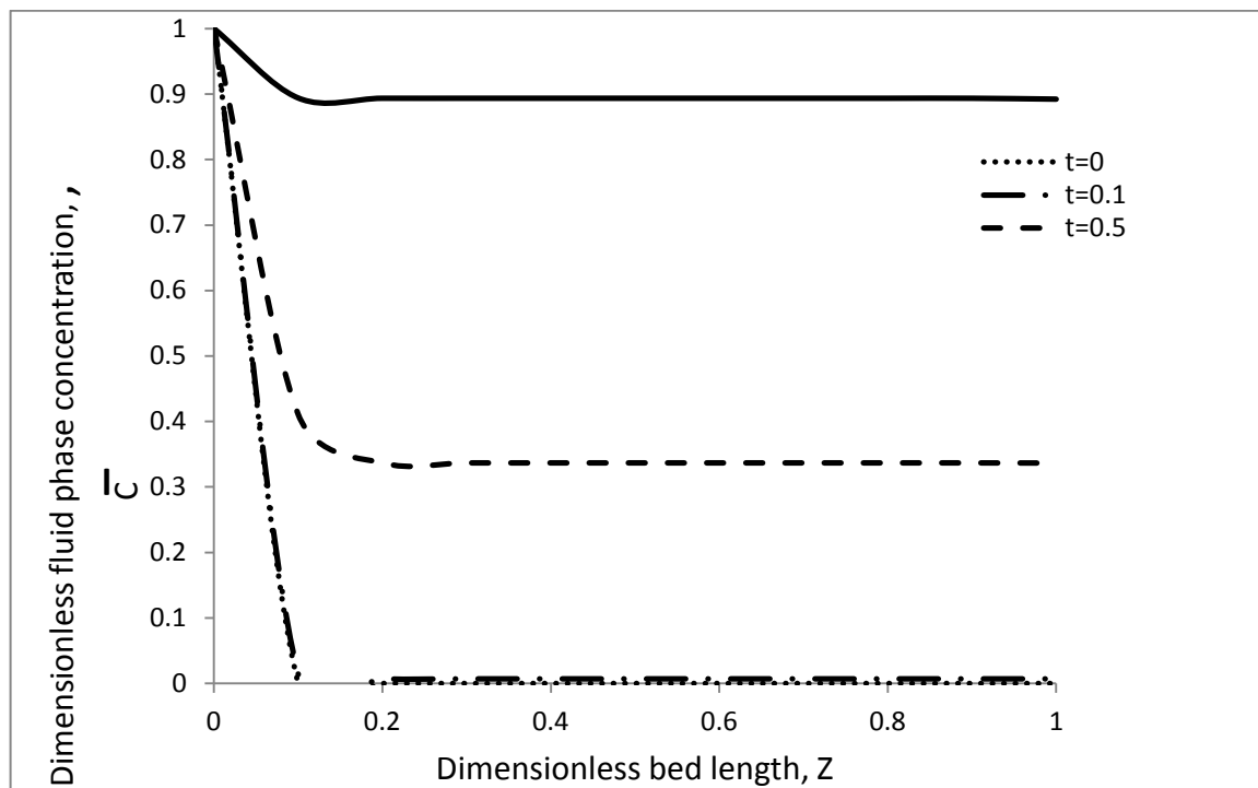
Figure 3. Plot of dimensionless fluid phase concentration of water against dimensionless bed length at different time
