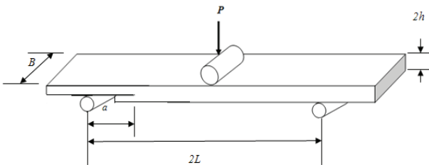
FIGURE 2 Schematic of test configuration for Mixed Mode Flexure Testing
