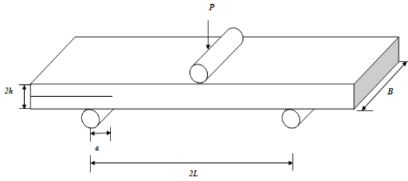
FIGURE 1 Schematic of the test configuration for the Mode II ENF Test.
