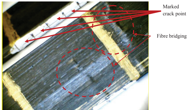
FIGURE 9 Photograph of a mixed-mode test specimen showing fibre bridging as the crack propagates from the initial crack to the mid span position.
