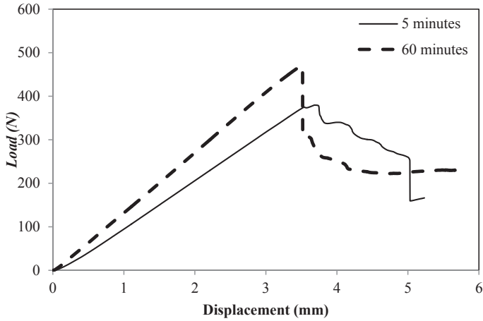
FIGURE 7 (b) Typical MMF load-displacement traces following processing at 300° with dwell times of 5 and 60 minutes.
