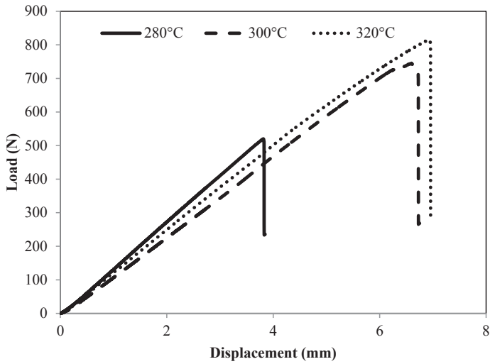
FIGURE 3 (b) Typical load-displacement traces, for Mode II samples processed at 280°C, 300°C and 320°C respectively with 5 minutes of dwell time.
