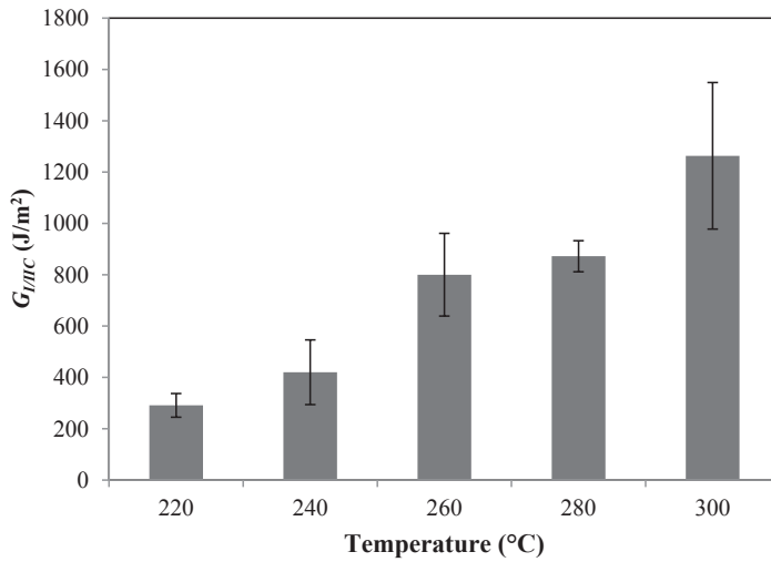
FIGURE 6 Plot of G_{I/IIc} at different processing temperatures for the Mixed-Mode fracture specimens manufactured using a dwell time of 5 minutes
