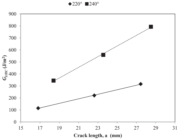
FIGURE 8 Representative R-curves for MMF test specimens processed at different processing temperatures, manufactured using a dwell time of 5 minutes.
