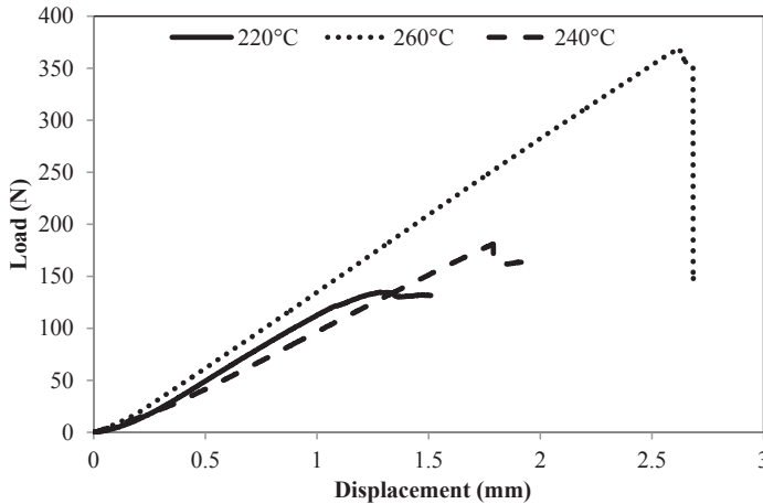
FIGURE 3 (a) Typical load-displacement traces for Mode II samples, processed at 220°C, 240°C and 260°C respectively with 5 minutes of dwell time.
