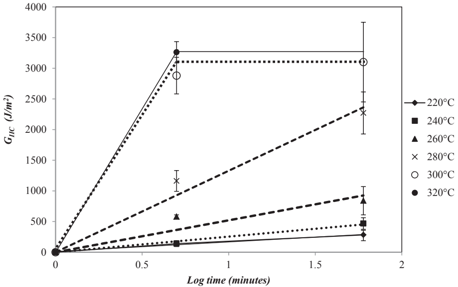
FIGURE 5 Plot of G_{IIC} versus Log time
