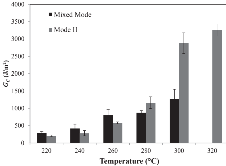
FIGURE 10 G_c versus processing temperature following both Mode II and Mixed-Mode I/II Interlaminar Fracture tests on specimens manufactured using a dwell time of 5 minutes.
