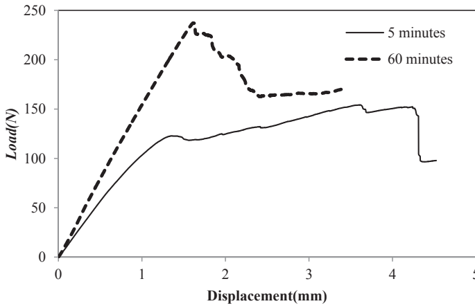
FIGURE 7 (a) Typical Mixed-Mode load-displacement traces following processing at 240°C with dwell times of 5 and 60 minutes.
