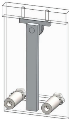
Figure 10. Pendulum-type switch developed for testing its feasibility
