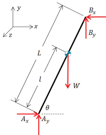
Figure 4. Free body diagram for the ladder Case I
