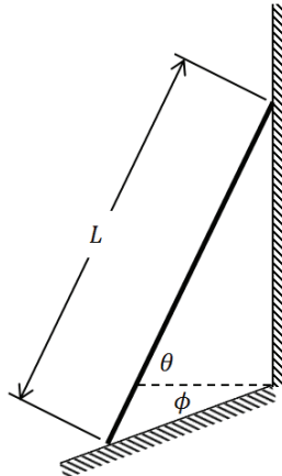
Figure 7. Setup of the ladder for Case III
