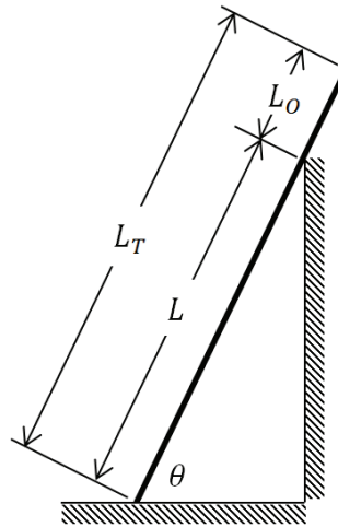
Figure 5. Setup of the ladder for Case II
