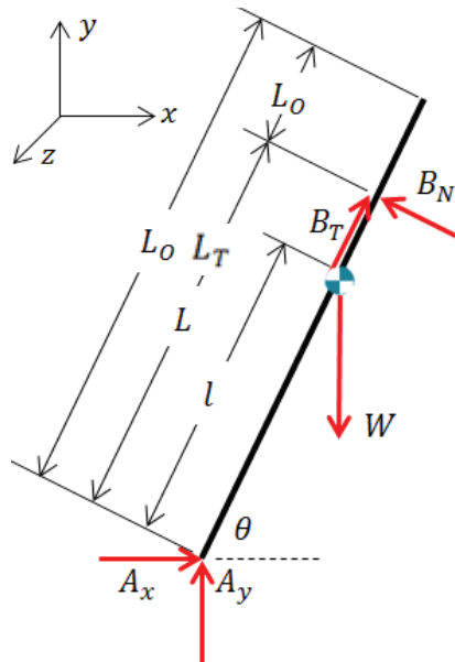
Figure 6. Free body diagram for the ladder in Case II
