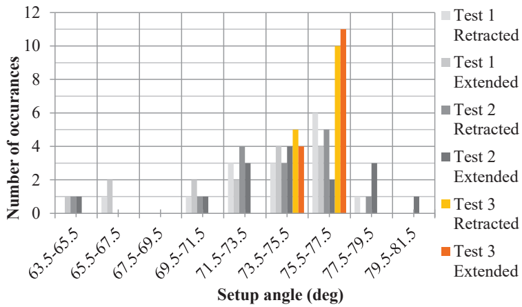
Figure 12. Distribution of the data from the test
