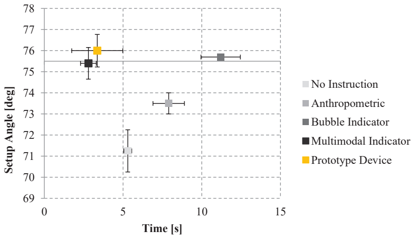
Figure 14. Setup time required for the prototype device compared to other ladder setup methods from previously published data (Simeonov, et al. 2013)
