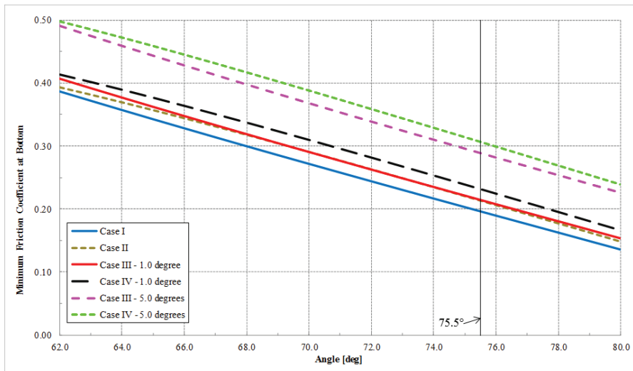
Figure 9. Plot comparing the minimum required friction at the base
