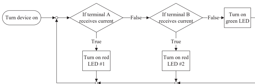
Figure 1. Switching logic
