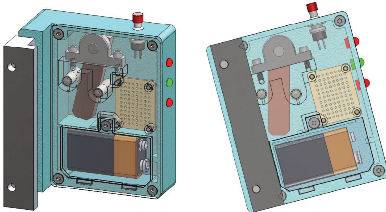
Figure 2. Mechanical design of the device
