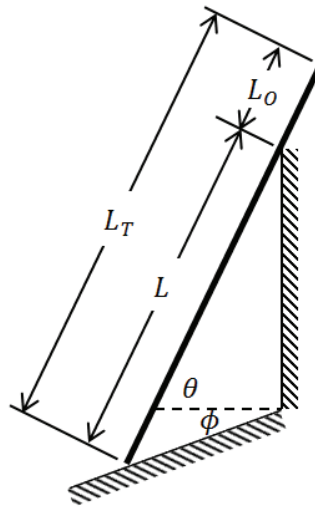
Figure 8. Setup of the ladder for Case IV
