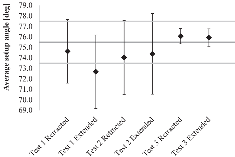
Figure 13. Results for the three tests, extended and retracted, with one standard deviate error bars
