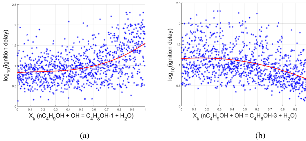
Figure 10. Component function for TRF/ n -butanol mixture at T = 761 K with respect to (a) n\text{-C}_4\text{H}_9\text{OH} + \text{OH} = \text{C}_4\text{H}_8\text{OH-1} + \text{H}_2\text{O} (b) n\text{-C}_4\text{H}_9\text{OH} + \text{OH} = \text{C}_4\text{H}_8\text{OH-3} + \text{H}_2\text{O} .
